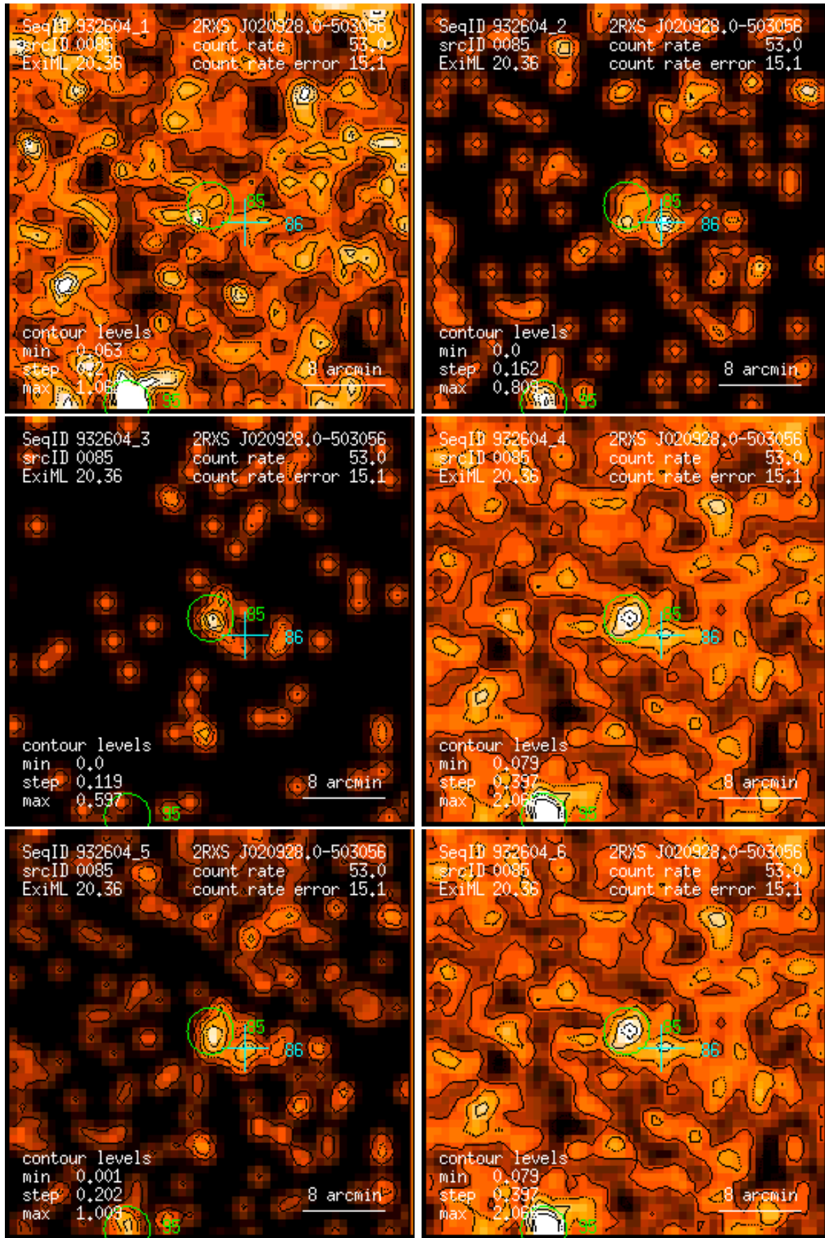
Figure 85: RASS 932604: detection 0085: band rate images, Gaussian filter: (1) PSPC channels 11 – 41, (2) 52 – 90, (3) 91 – 201, (4) 11 – 235, (5) 52 – 201, (6) 11 – 201. Broad band rates in counts/ks. Band rate contour levels in counts/ks/arcmin 2 .
