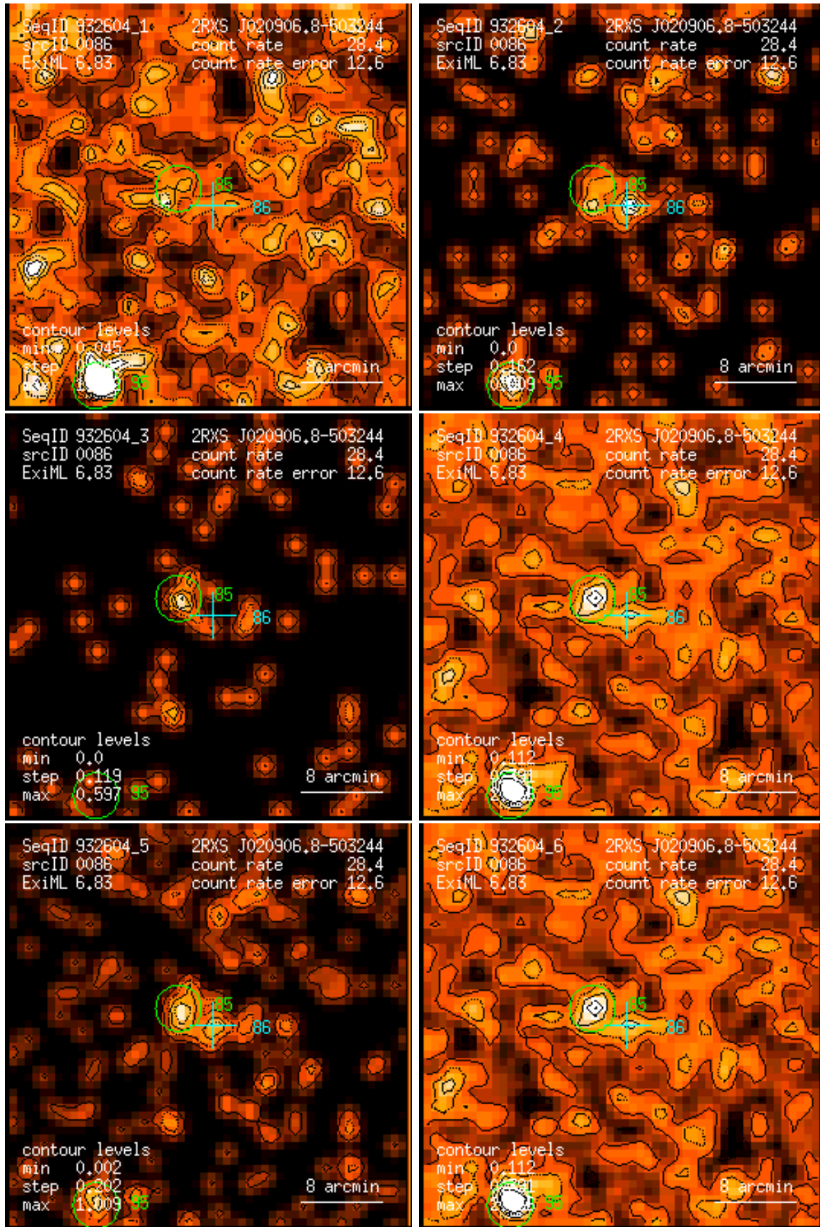
Figure 86: RASS 932604: detection 0086: band rate images, Gaussian filter: (1) PSPC channels 11 – 41, (2) 52 – 90, (3) 91 – 201, (4) 11 – 235, (5) 52 – 201, (6) 11 – 201. Broad band rates in counts/ks. Band rate contour levels in counts/ks/arcmin 2 .
