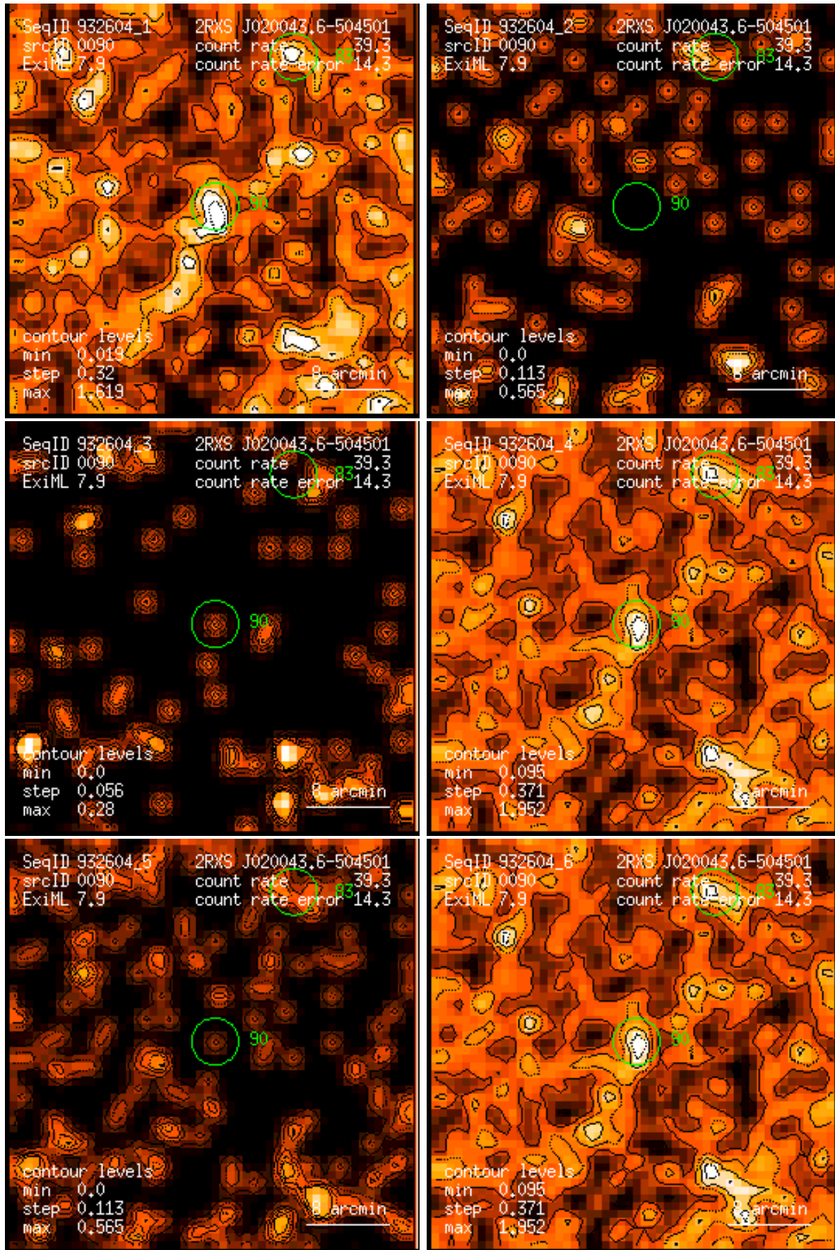
Figure 90: RASS 932604: detection 0090: band rate images, Gaussian filter: (1) PSPC channels 11 – 41, (2) 52 – 90, (3) 91 – 201, (4) 11 – 235, (5) 52 – 201, (6) 11 – 201. Broad band rates in counts/ks. Band rate contour levels in counts/ks/arcmin 2 .
