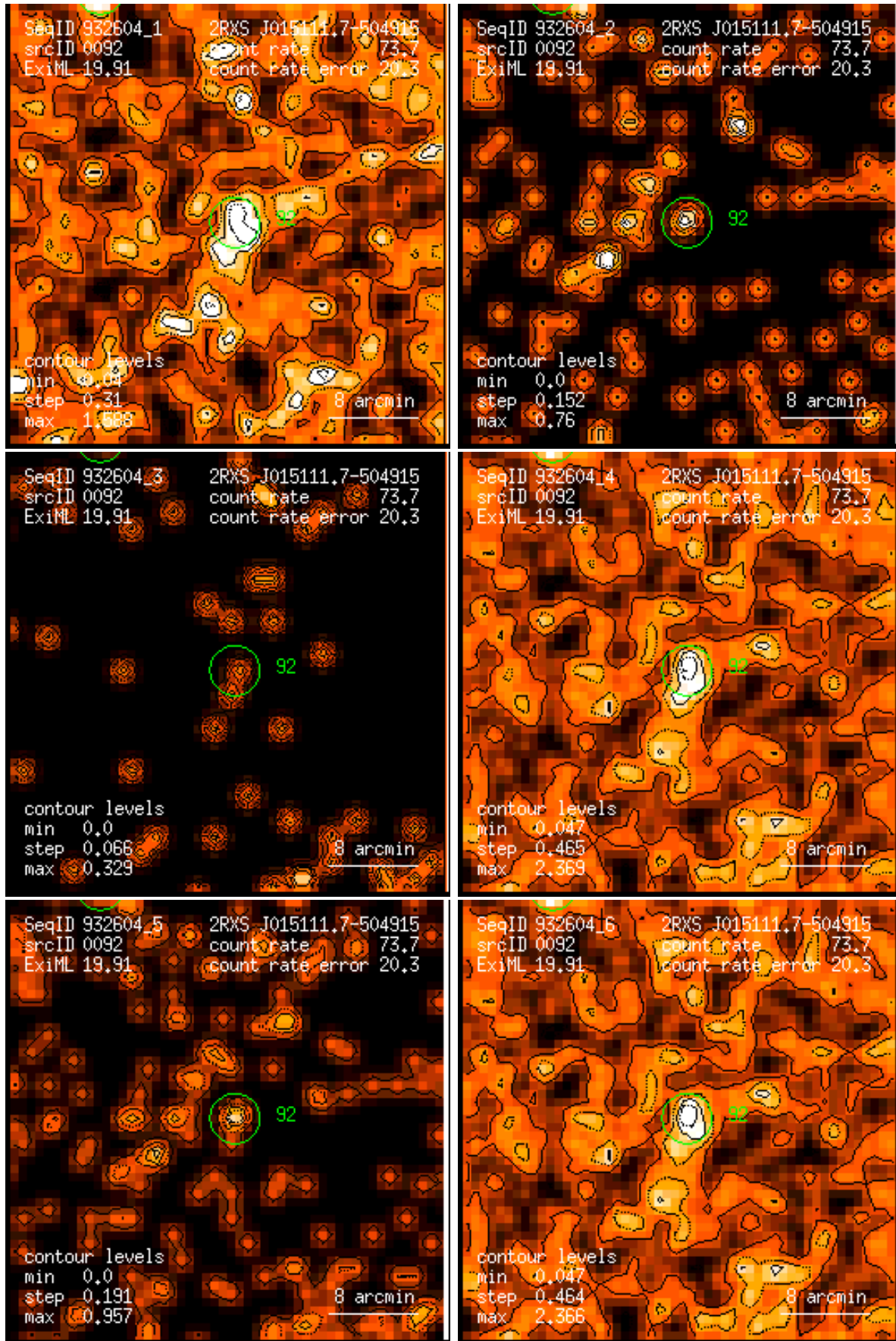
Figure 92: RASS 932604: detection 0092: band rate images, Gaussian filter: (1) PSPC channels 11 – 41, (2) 52 – 90, (3) 91 – 201, (4) 11 – 235, (5) 52 – 201, (6) 11 – 201. Broad band rates in counts/ks. Band rate contour levels in counts/ks/arcmin 2 .
