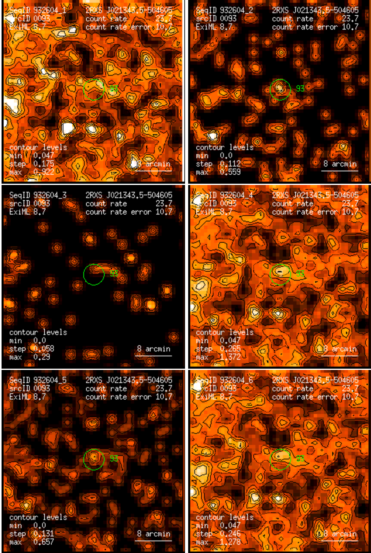
Figure 93: RASS 932604: detection 0093: band rate images, Gaussian filter: (1) PSPC channels 11 – 41, (2) 52 – 90, (3) 91 – 201, (4) 11 – 235, (5) 52 – 201, (6) 11 – 201. Broad band rates in counts/ks. Band rate contour levels in counts/ks/arcmin 2 .
