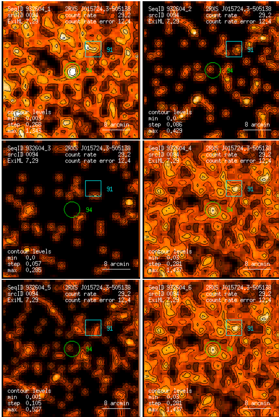
Figure 94: RASS 932604: detection 0094: band rate images, Gaussian filter: (1) PSPC channels 11 – 41, (2) 52 – 90, (3) 91 – 201, (4) 11 – 235, (5) 52 – 201, (6) 11 – 201. Broad band rates in counts/ks. Band rate contour levels in counts/ks/arcmin 2 .
