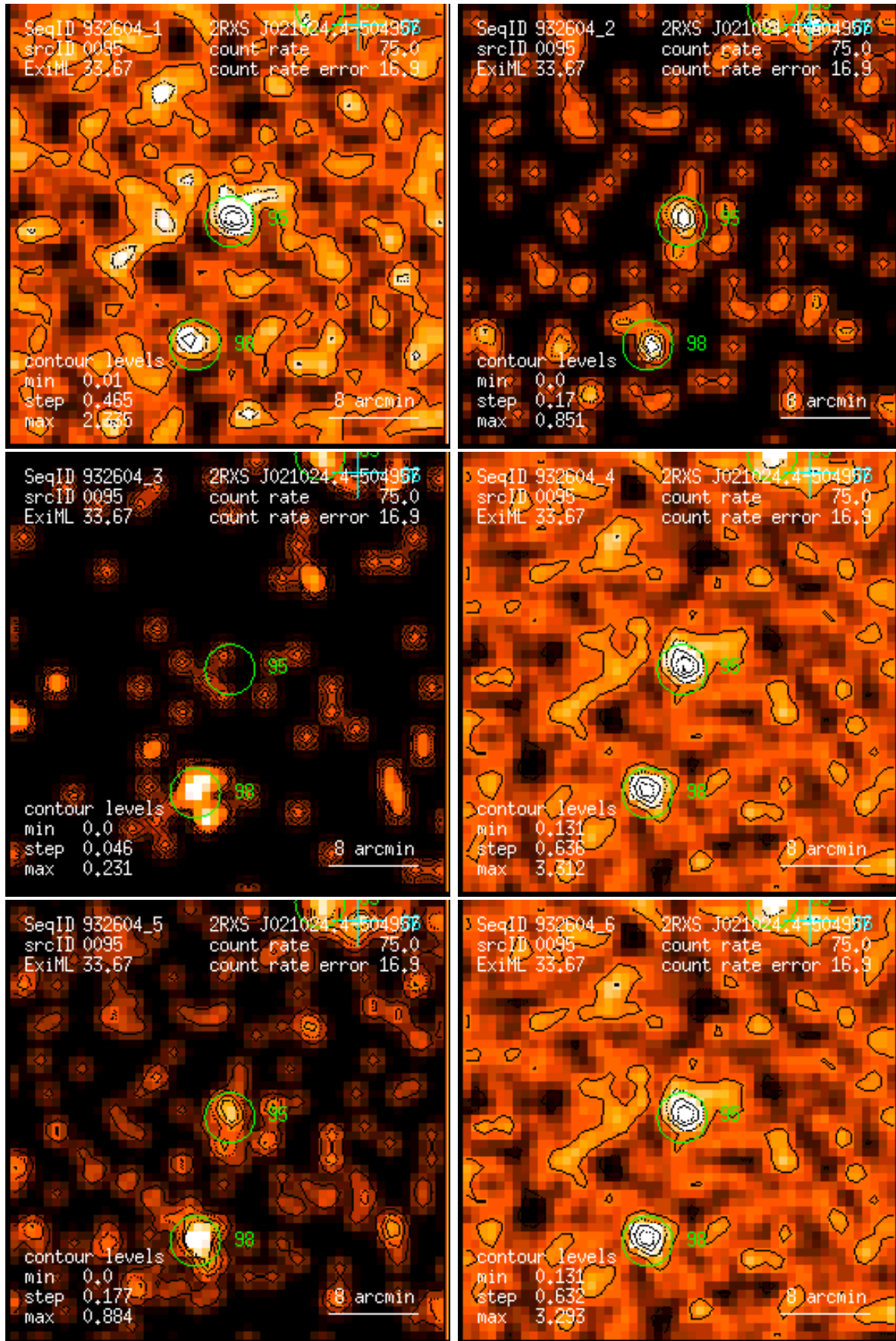
Figure 95: RASS 932604: detection 0095: band rate images, Gaussian filter: (1) PSPC channels 11 – 41, (2) 52 – 90, (3) 91 – 201, (4) 11 – 235, (5) 52 – 201, (6) 11 – 201. Broad band rates in counts/ks. Band rate contour levels in counts/ks/arcmin 2 .
