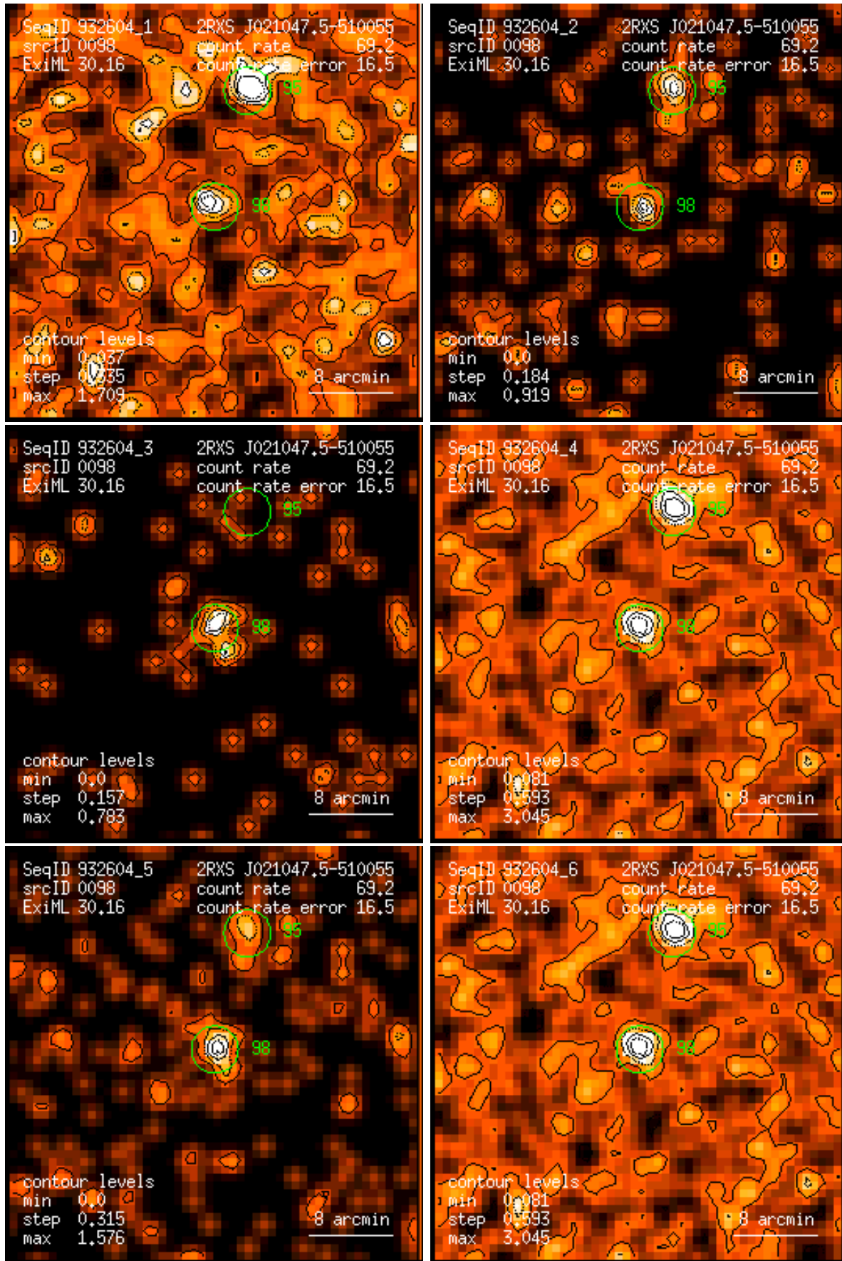
Figure 98: RASS 932604: detection 0098: band rate images, Gaussian filter: (1) PSPC channels 11 – 41, (2) 52 – 90, (3) 91 – 201, (4) 11 – 235, (5) 52 – 201, (6) 11 – 201. Broad band rates in counts/ks. Band rate contour levels in counts/ks/arcmin 2 .
