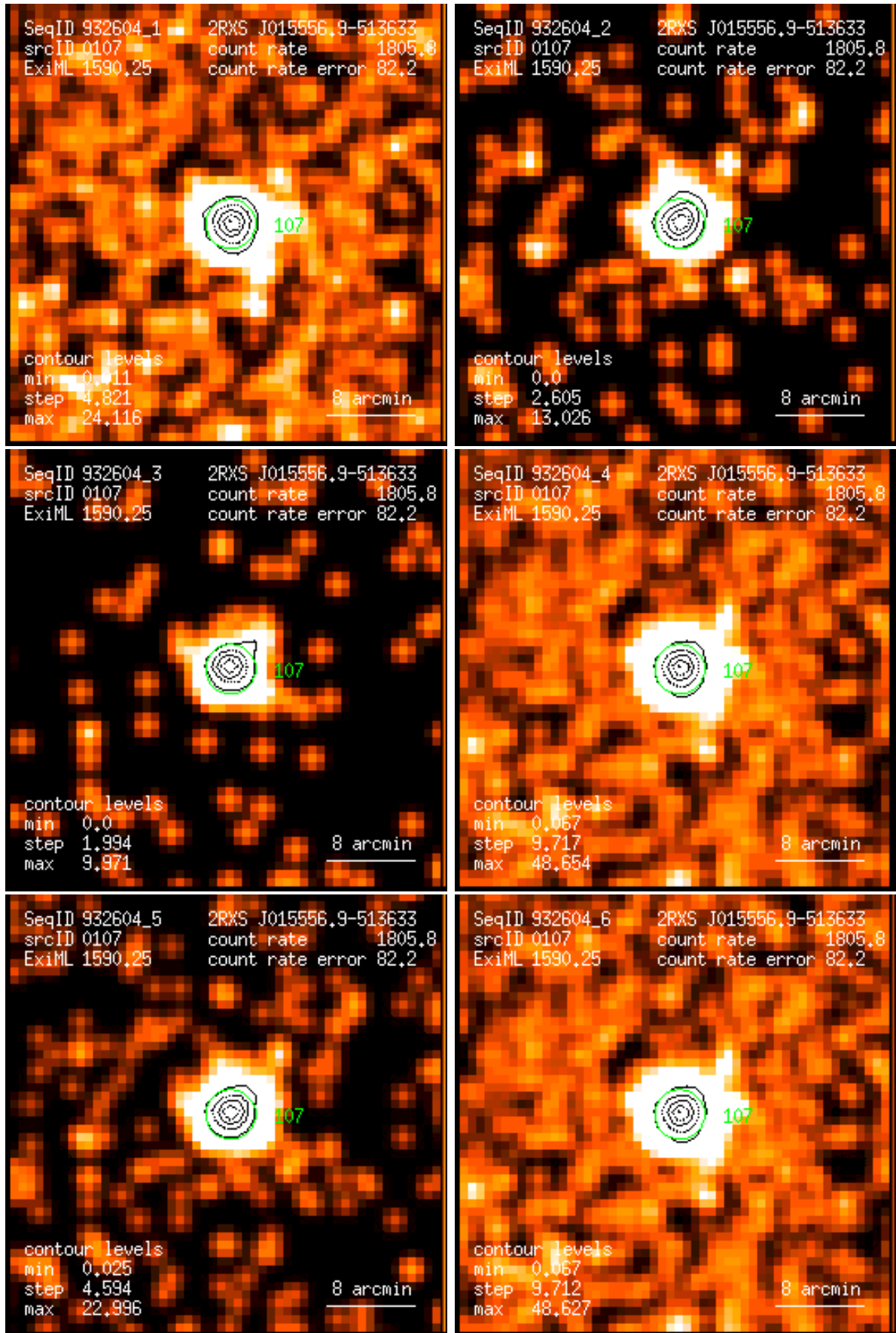
Figure 107: RASS 932604: detection 0107: band rate images, Gaussian filter: (1) PSPC channels 11 – 41, (2) 52 – 90, (3) 91 – 201, (4) 11 – 235, (5) 52 – 201, (6) 11 – 201. Broad band rates in counts/ks. Band rate contour levels in counts/ks/arcmin 2 .
