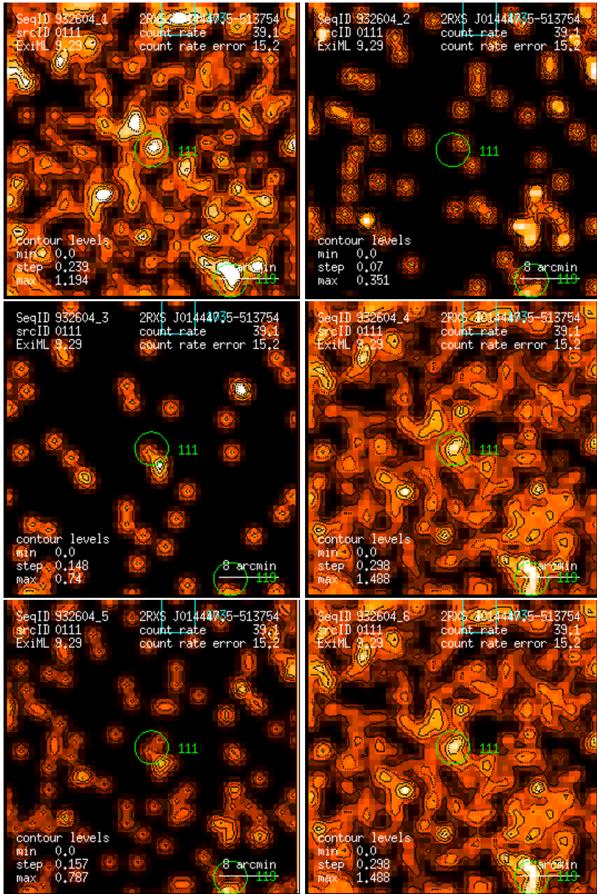
Figure 111: RASS 932604: detection 0111: band rate images, Gaussian filter: (1) PSPC channels 11 – 41, (2) 52 – 90, (3) 91 – 201, (4) 11 – 235, (5) 52 – 201, (6) 11 – 201. Broad band rates in counts/ks. Band rate contour levels in counts/ks/arcmin 2 .
