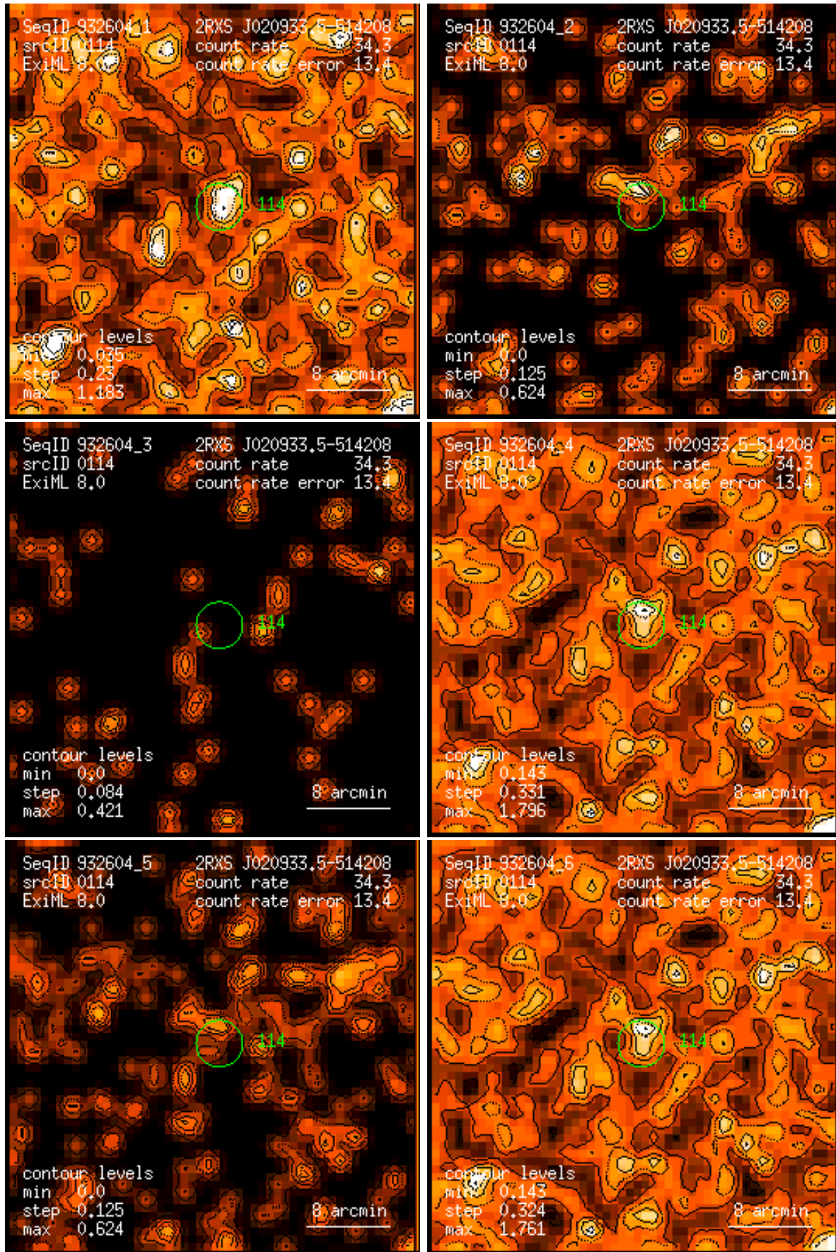
Figure 114: RASS 932604: detection 0114: band rate images, Gaussian filter: (1) PSPC channels 11 – 41, (2) 52 – 90, (3) 91 – 201, (4) 11 – 235, (5) 52 – 201, (6) 11 – 201. Broad band rates in counts/ks. Band rate contour levels in counts/ks/arcmin 2 .
