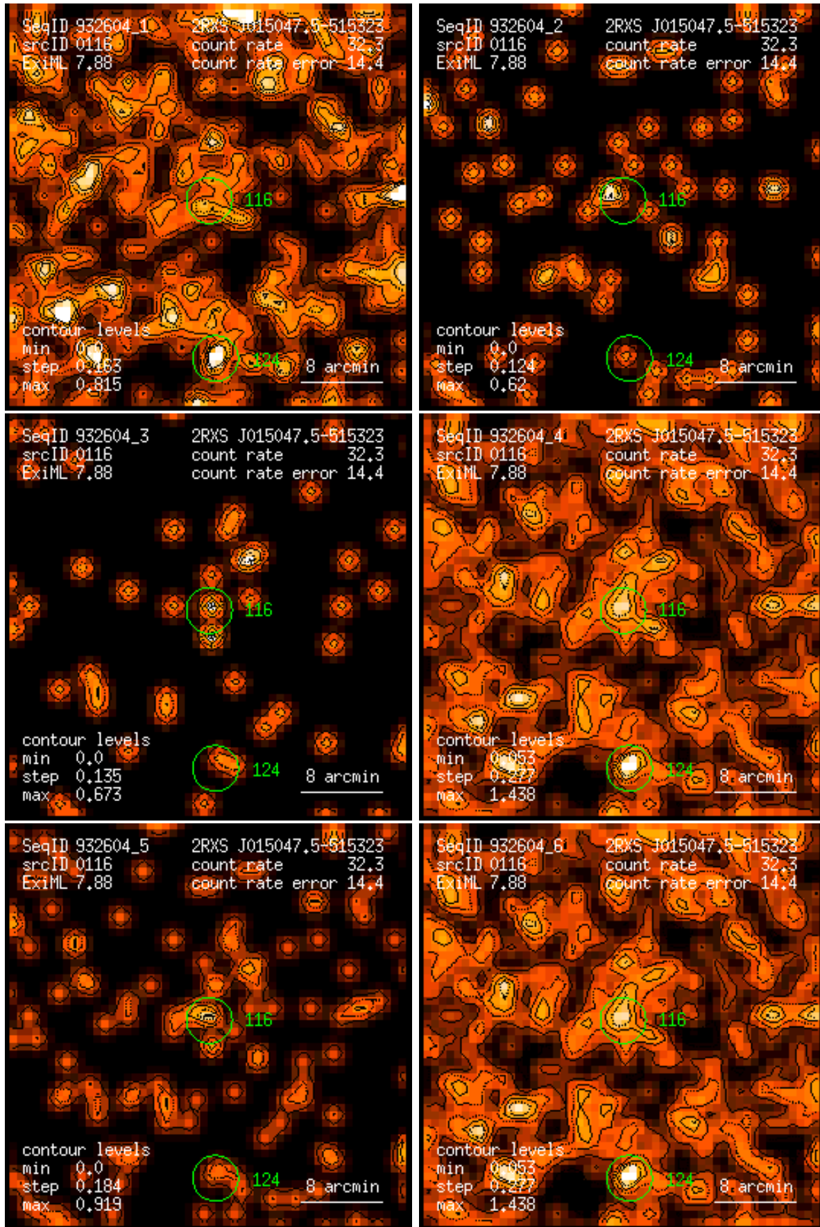
Figure 116: RASS 932604: detection 0116: band rate images, Gaussian filter: (1) PSPC channels 11 – 41, (2) 52 – 90, (3) 91 – 201, (4) 11 – 235, (5) 52 – 201, (6) 11 – 201. Broad band rates in counts/ks. Band rate contour levels in counts/ks/arcmin 2 .
