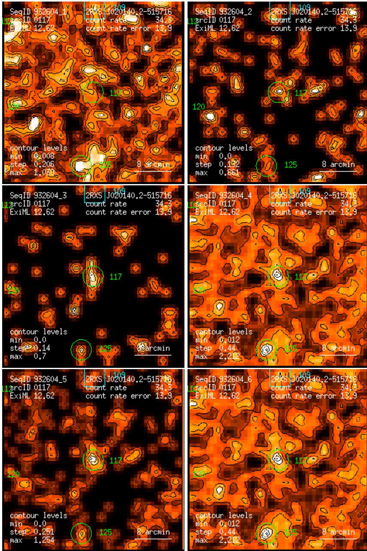
Figure 117: RASS 932604: detection 0117: band rate images, Gaussian filter: (1) PSPC channels 11 – 41, (2) 52 – 90, (3) 91 – 201, (4) 11 – 235, (5) 52 – 201, (6) 11 – 201. Broad band rates in counts/ks. Band rate contour levels in counts/ks/arcmin 2 .
