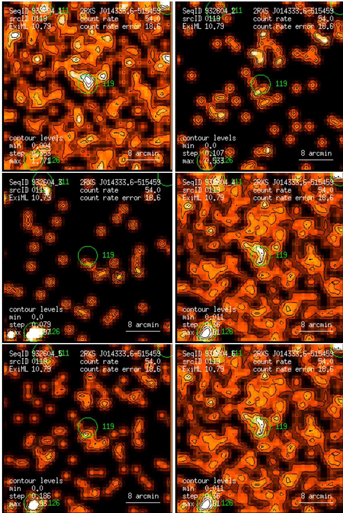
Figure 119: RASS 932604: detection 0119: band rate images, Gaussian filter: (1) PSPC channels 11 – 41, (2) 52 – 90, (3) 91 – 201, (4) 11 – 235, (5) 52 – 201, (6) 11 – 201. Broad band rates in counts/ks. Band rate contour levels in counts/ks/arcmin 2 .
