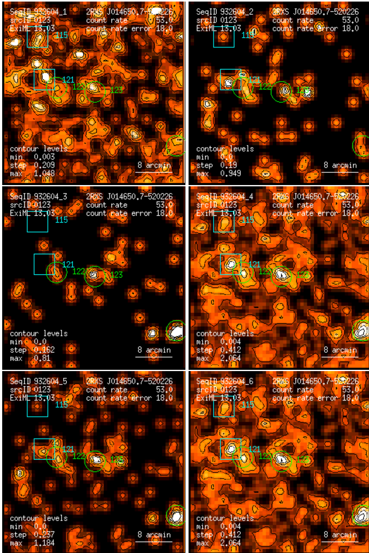
Figure 123: RASS 932604: detection 0123: band rate images, Gaussian filter: (1) PSPC channels 11 – 41, (2) 52 – 90, (3) 91 – 201, (4) 11 – 235, (5) 52 – 201, (6) 11 – 201. Broad band rates in counts/ks. Band rate contour levels in counts/ks/arcmin 2 .
