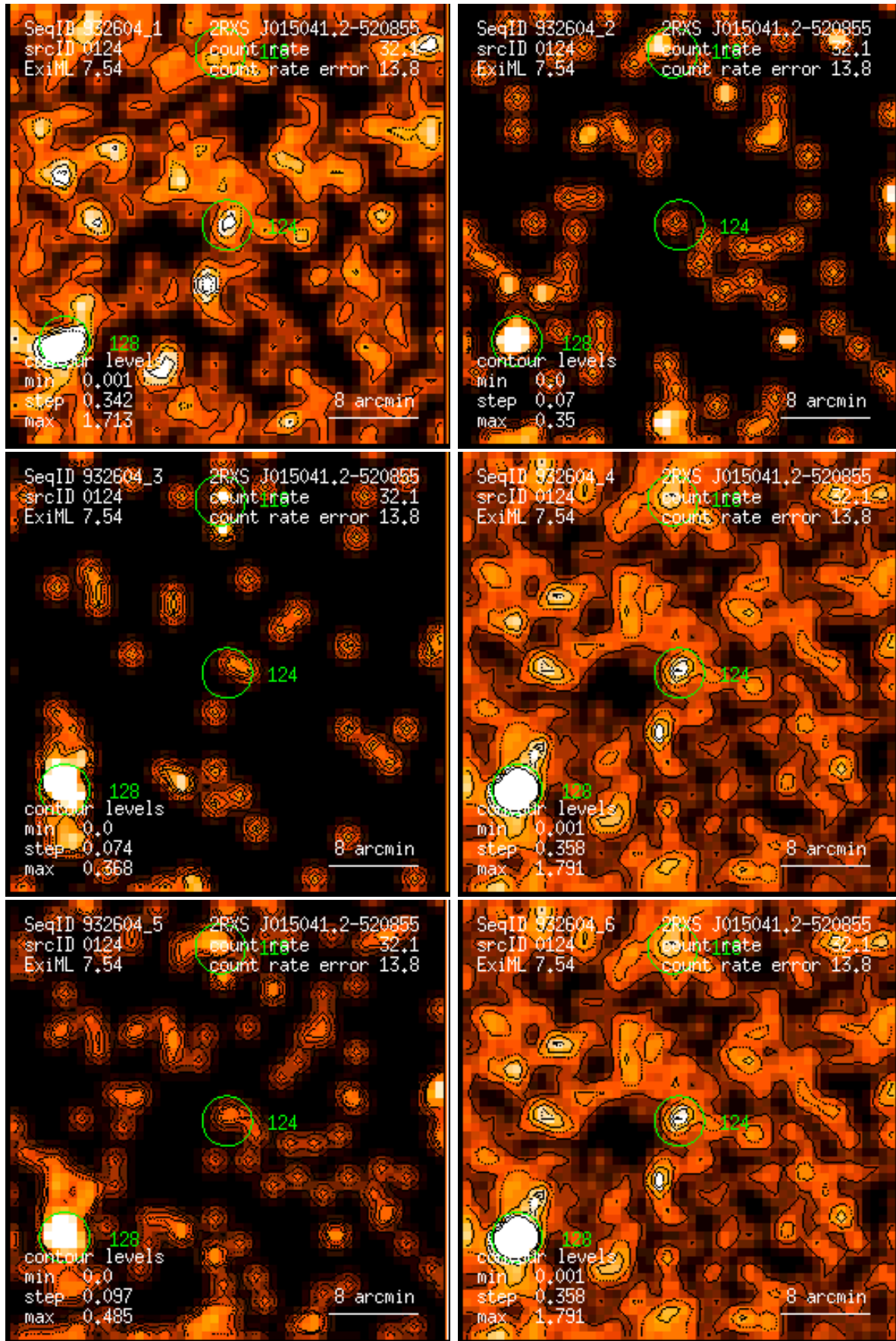
Figure 124: RASS 932604: detection 0124: band rate images, Gaussian filter: (1) PSPC channels 11 – 41, (2) 52 – 90, (3) 91 – 201, (4) 11 – 235, (5) 52 – 201, (6) 11 – 201. Broad band rates in counts/ks. Band rate contour levels in counts/ks/arcmin 2 .
