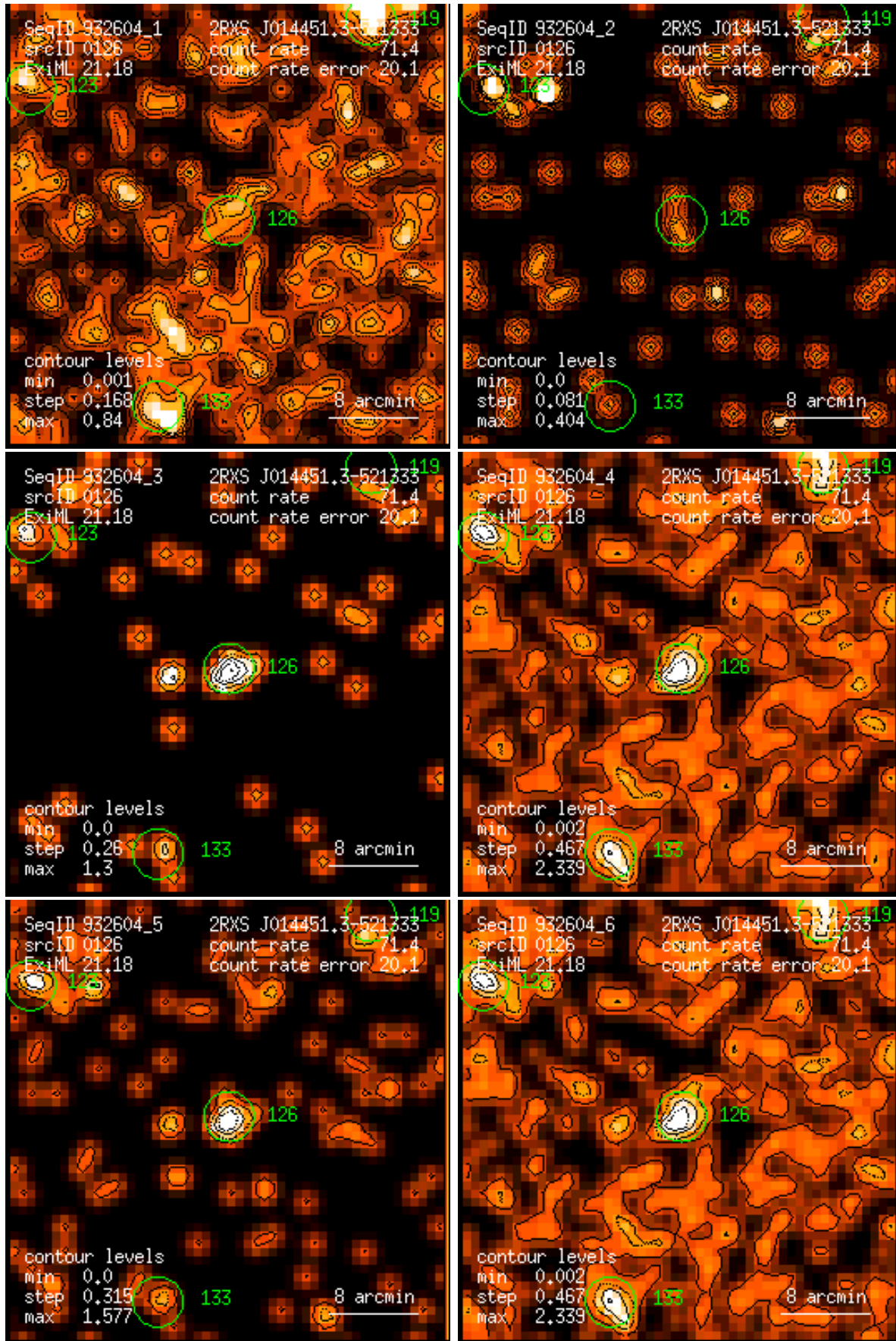
Figure 126: RASS 932604: detection 0126: band rate images, Gaussian filter: (1) PSPC channels 11 – 41, (2) 52 – 90, (3) 91 – 201, (4) 11 – 235, (5) 52 – 201, (6) 11 – 201. Broad band rates in counts/ks. Band rate contour levels in counts/ks/arcmin 2 .
