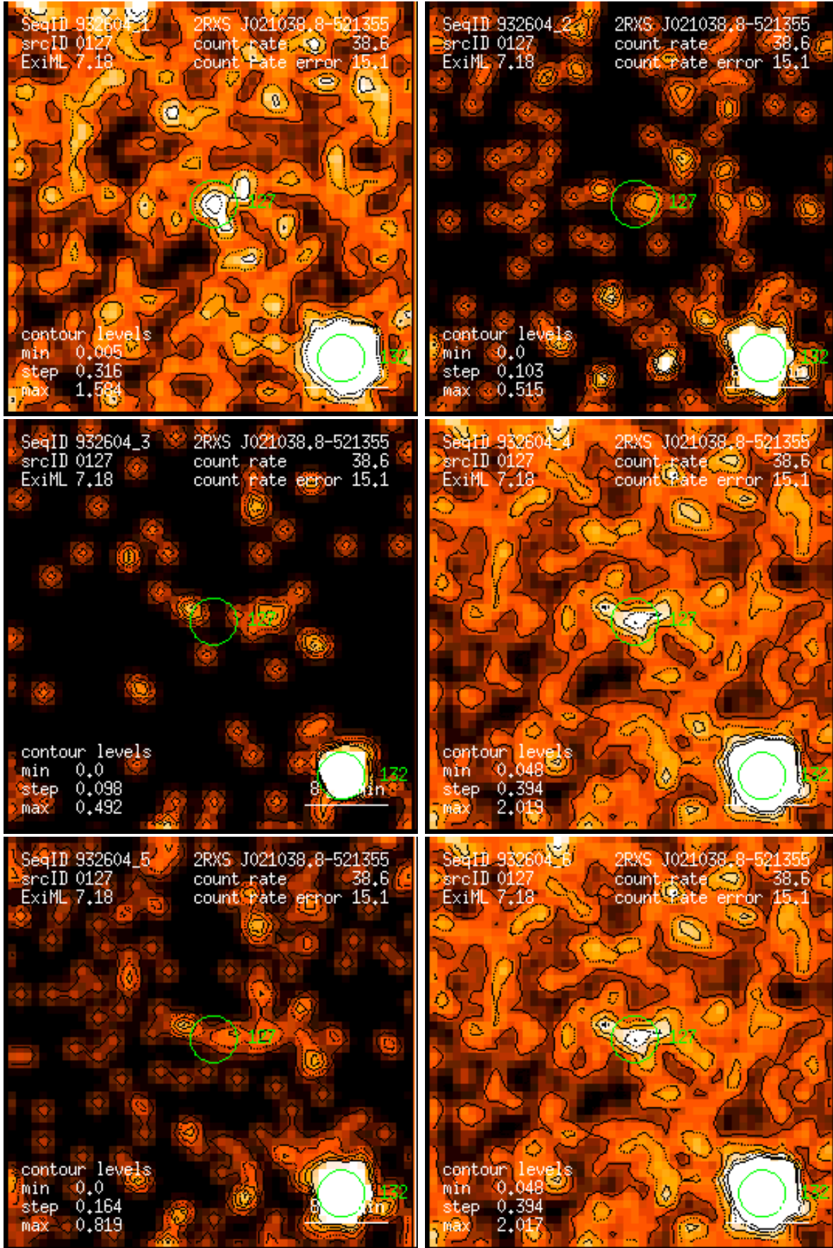
Figure 127: RASS 932604: detection 0127: band rate images, Gaussian filter: (1) PSPC channels 11 – 41, (2) 52 – 90, (3) 91 – 201, (4) 11 – 235, (5) 52 – 201, (6) 11 – 201. Broad band rates in counts/ks. Band rate contour levels in counts/ks/arcmin 2 .
