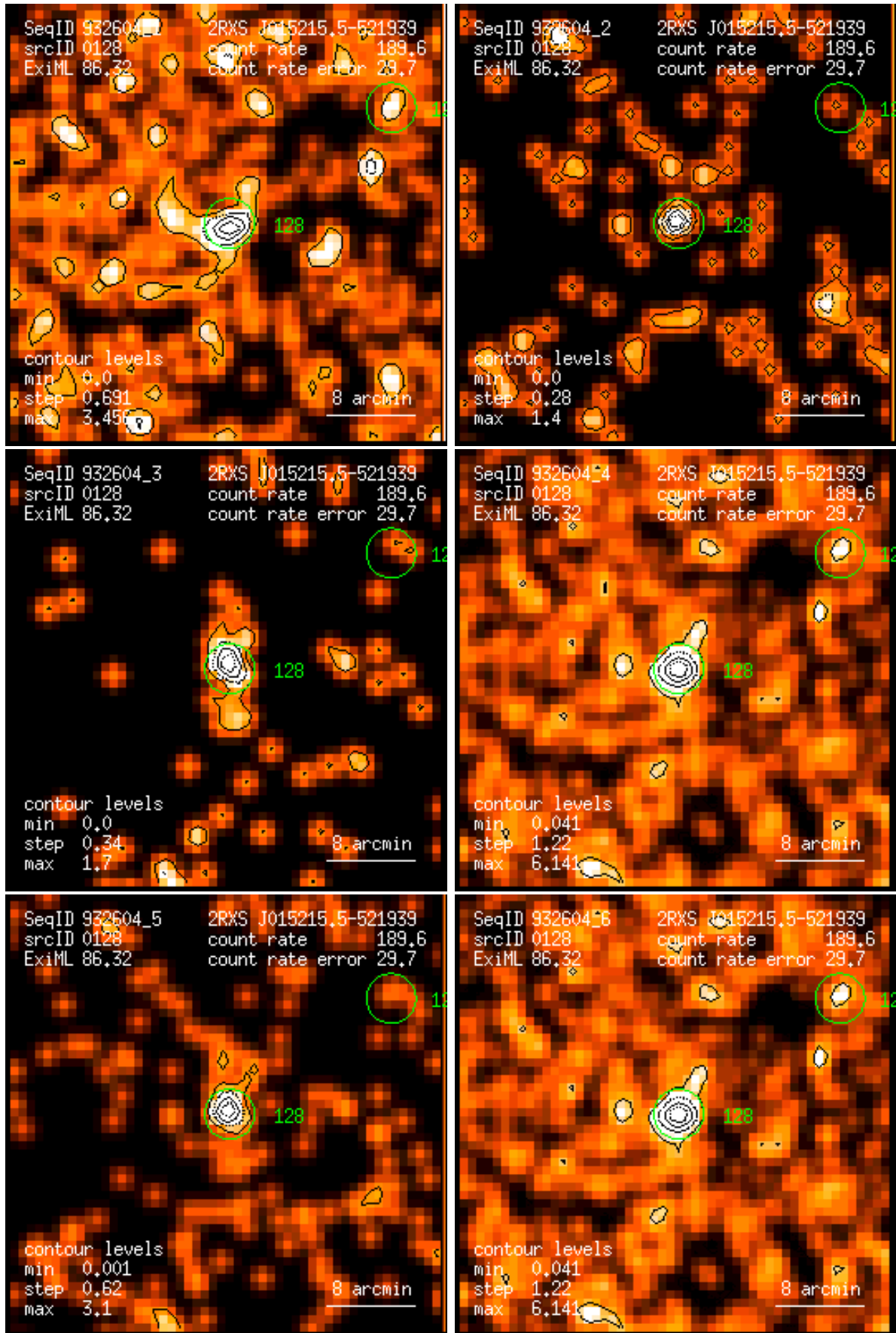
Figure 128: RASS 932604: detection 0128: band rate images, Gaussian filter: (1) PSPC channels 11 – 41, (2) 52 – 90, (3) 91 – 201, (4) 11 – 235, (5) 52 – 201, (6) 11 – 201. Broad band rates in counts/ks. Band rate contour levels in counts/ks/arcmin 2 .
