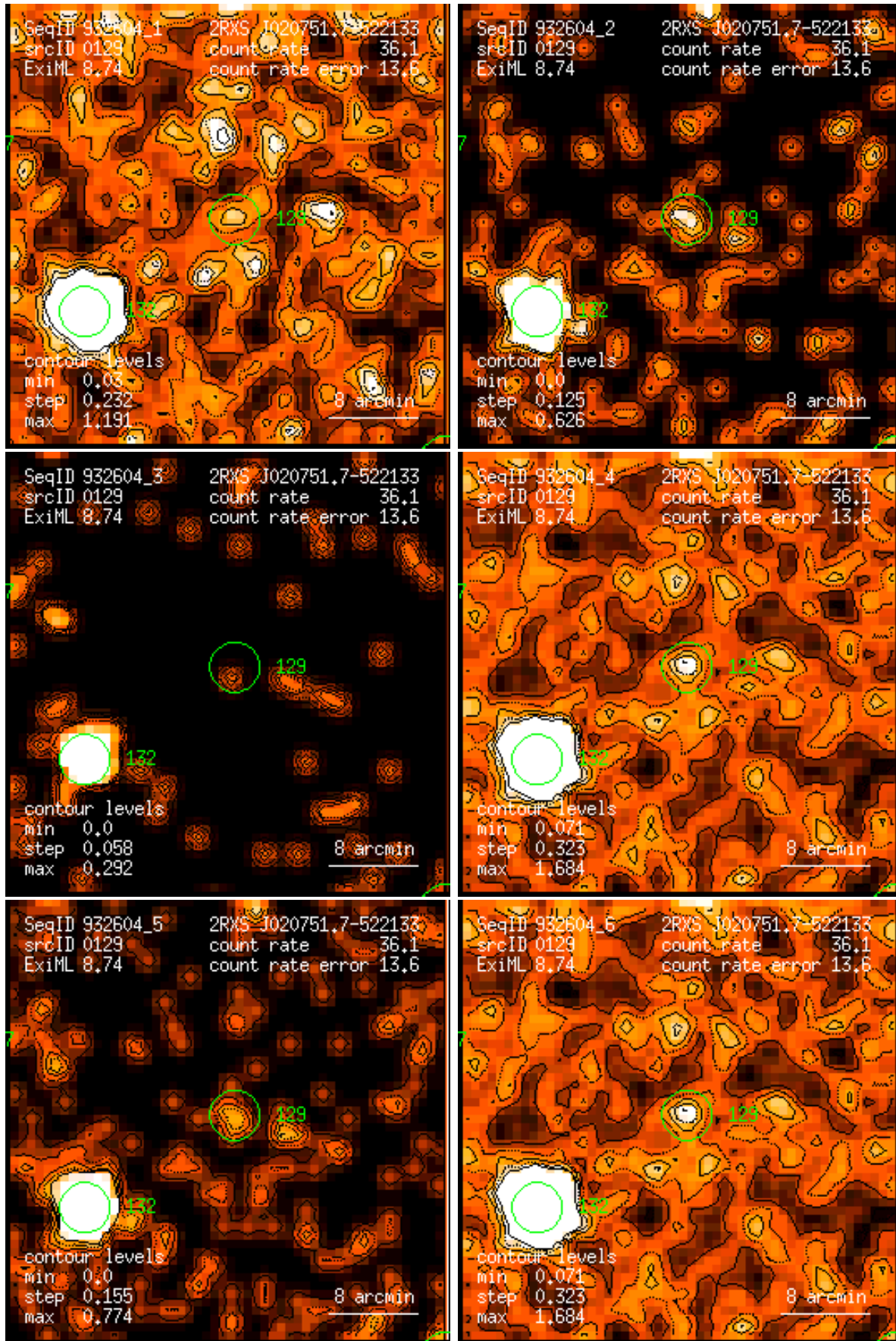
Figure 129: RASS 932604: detection 0129: band rate images, Gaussian filter: (1) PSPC channels 11 – 41, (2) 52 – 90, (3) 91 – 201, (4) 11 – 235, (5) 52 – 201, (6) 11 – 201. Broad band rates in counts/ks. Band rate contour levels in counts/ks/arcmin 2 .
