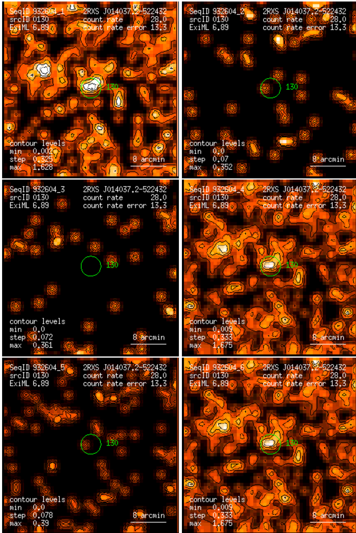
Figure 130: RASS 932604: detection 0130: band rate images, Gaussian filter: (1) PSPC channels 11 – 41, (2) 52 – 90, (3) 91 – 201, (4) 11 – 235, (5) 52 – 201, (6) 11 – 201. Broad band rates in counts/ks. Band rate contour levels in counts/ks/arcmin 2 .
