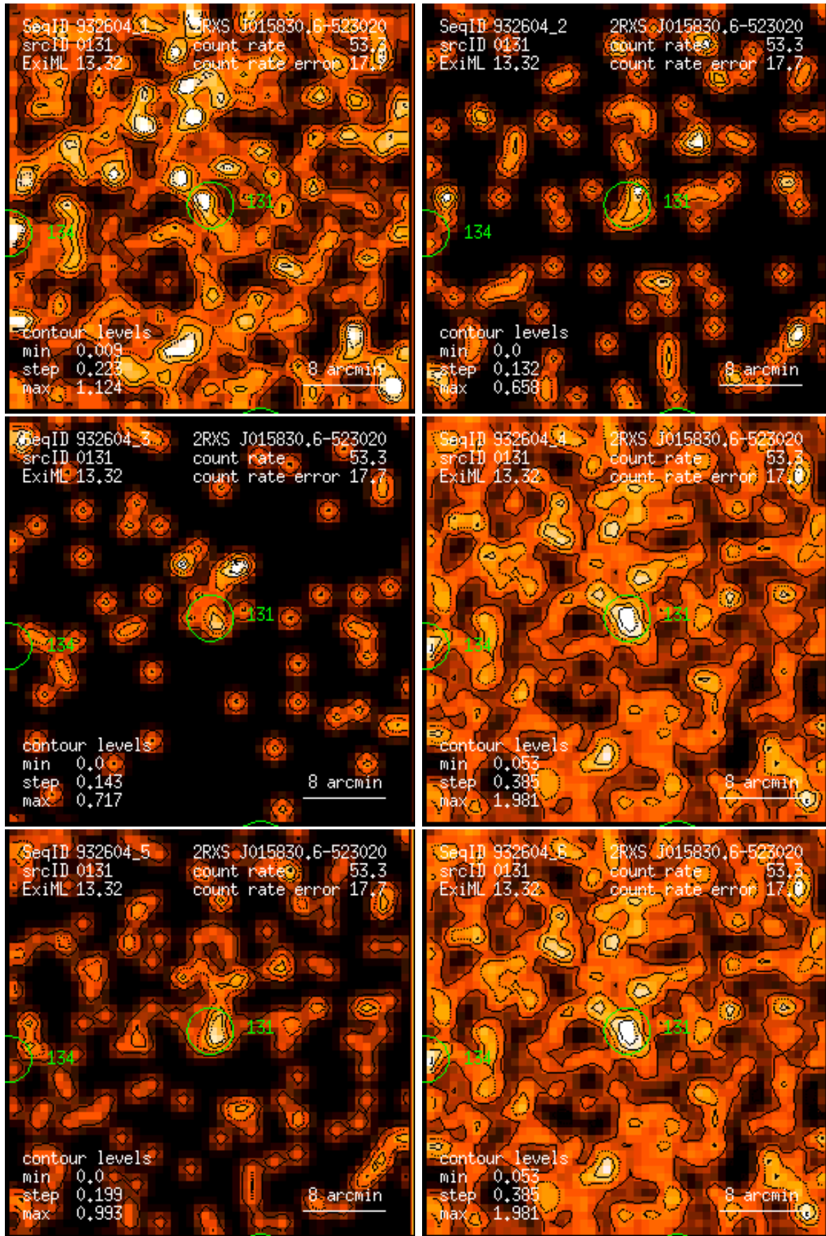
Figure 131: RASS 932604: detection 0131: band rate images, Gaussian filter: (1) PSPC channels 11 – 41, (2) 52 – 90, (3) 91 – 201, (4) 11 – 235, (5) 52 – 201, (6) 11 – 201. Broad band rates in counts/ks. Band rate contour levels in counts/ks/arcmin 2 .
