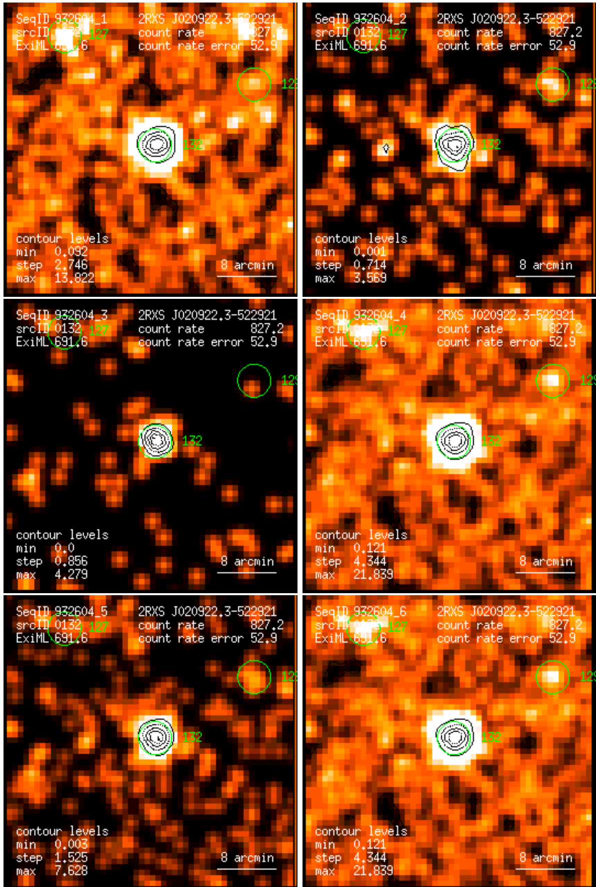
Figure 132: RASS 932604: detection 0132: band rate images, Gaussian filter: (1) PSPC channels 11 – 41, (2) 52 – 90, (3) 91 – 201, (4) 11 – 235, (5) 52 – 201, (6) 11 – 201. Broad band rates in counts/ks. Band rate contour levels in counts/ks/arcmin 2 .
