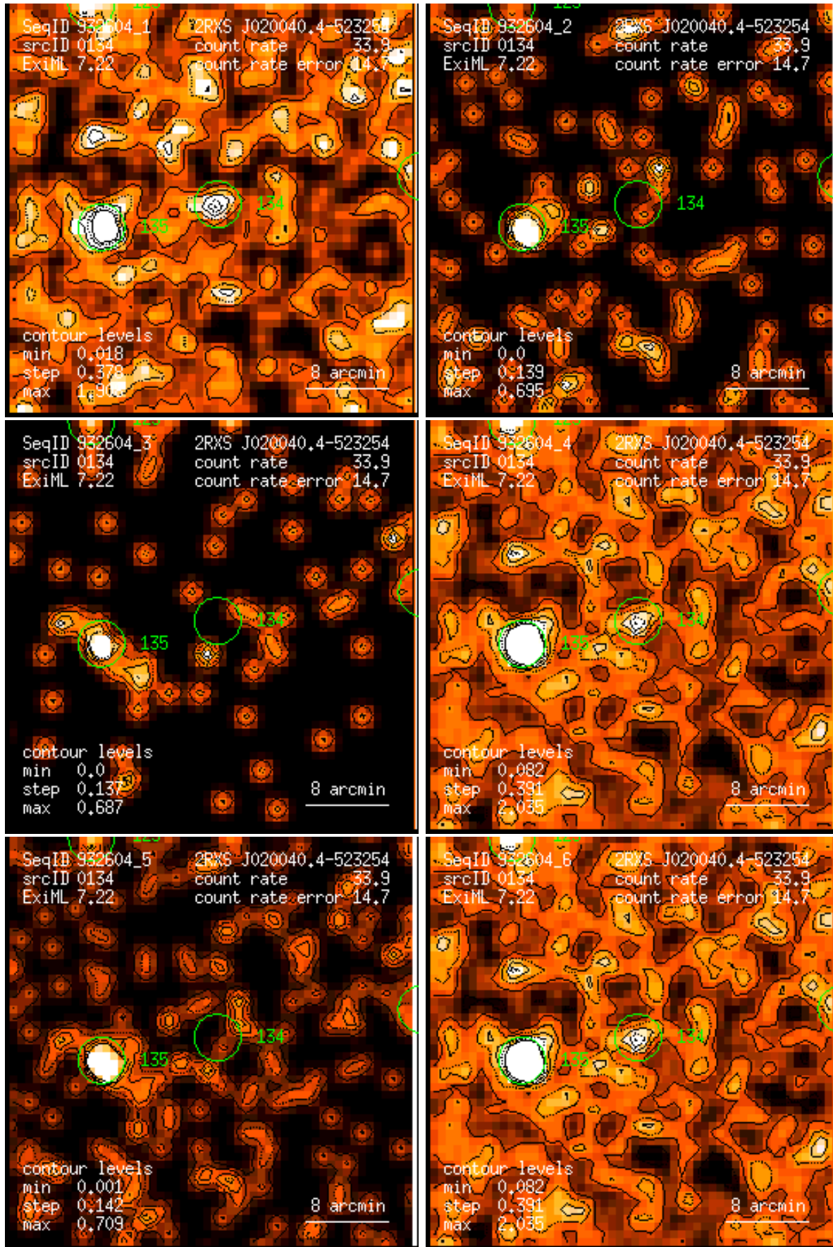
Figure 134: RASS 932604: detection 0134: band rate images, Gaussian filter: (1) PSPC channels 11 – 41, (2) 52 – 90, (3) 91 – 201, (4) 11 – 235, (5) 52 – 201, (6) 11 – 201. Broad band rates in counts/ks. Band rate contour levels in counts/ks/arcmin 2 .
