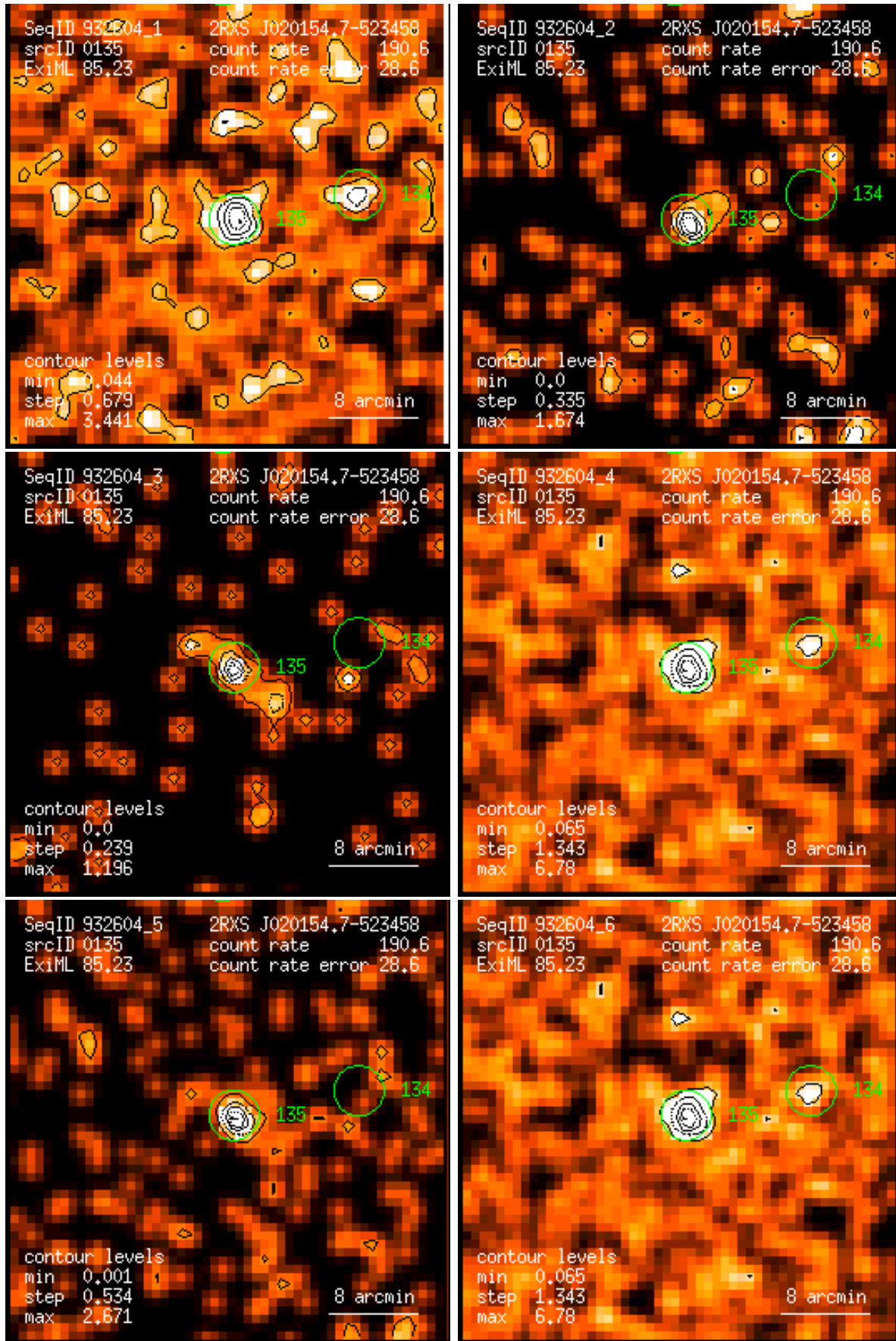
Figure 135: RASS 932604: detection 0135: band rate images, Gaussian filter: (1) PSPC channels 11 – 41, (2) 52 – 90, (3) 91 – 201, (4) 11 – 235, (5) 52 – 201, (6) 11 – 201. Broad band rates in counts/ks. Band rate contour levels in counts/ks/arcmin 2 .
