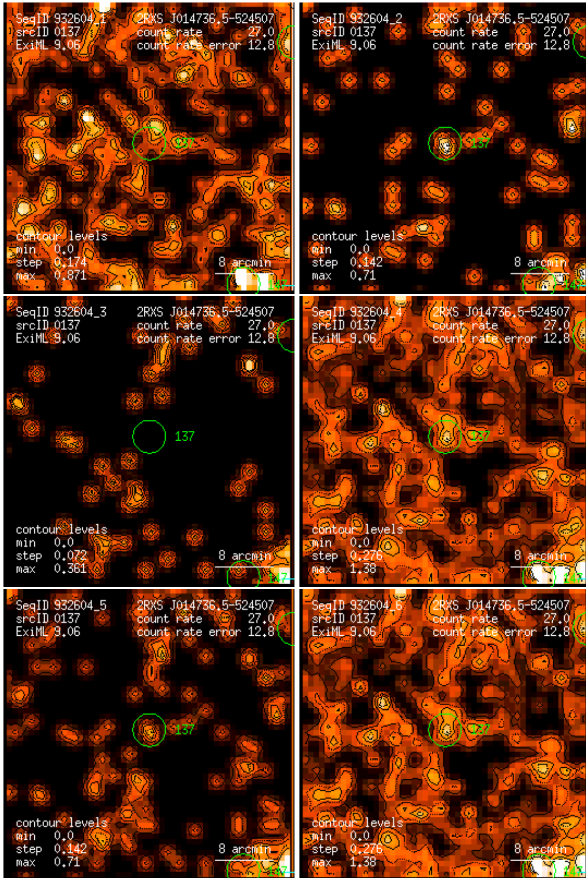
Figure 137: RASS 932604: detection 0137: band rate images, Gaussian filter: (1) PSPC channels 11 – 41, (2) 52 – 90, (3) 91 – 201, (4) 11 – 235, (5) 52 – 201, (6) 11 – 201. Broad band rates in counts/ks. Band rate contour levels in counts/ks/arcmin 2 .
