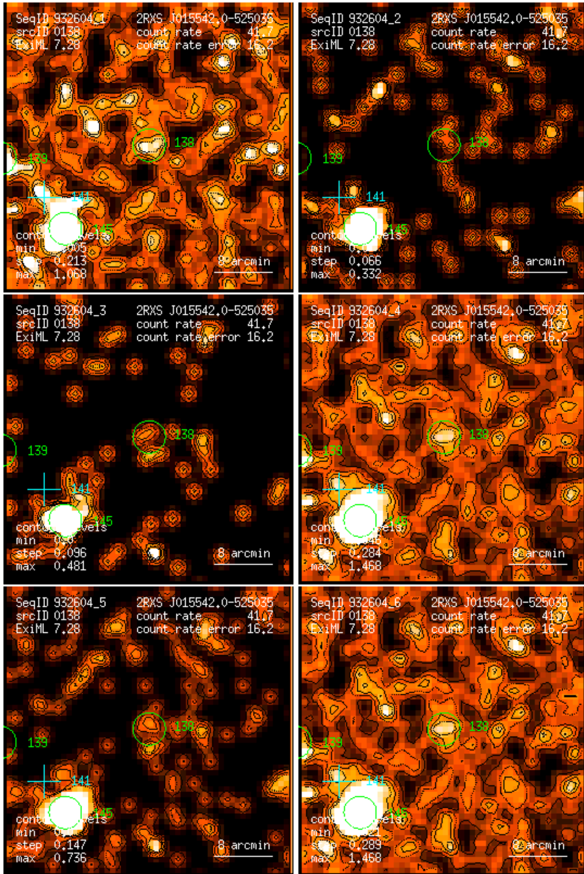
Figure 138: RASS 932604: detection 0138: band rate images, Gaussian filter: (1) PSPC channels 11 – 41, (2) 52 – 90, (3) 91 – 201, (4) 11 – 235, (5) 52 – 201, (6) 11 – 201. Broad band rates in counts/ks. Band rate contour levels in counts/ks/arcmin 2 .
