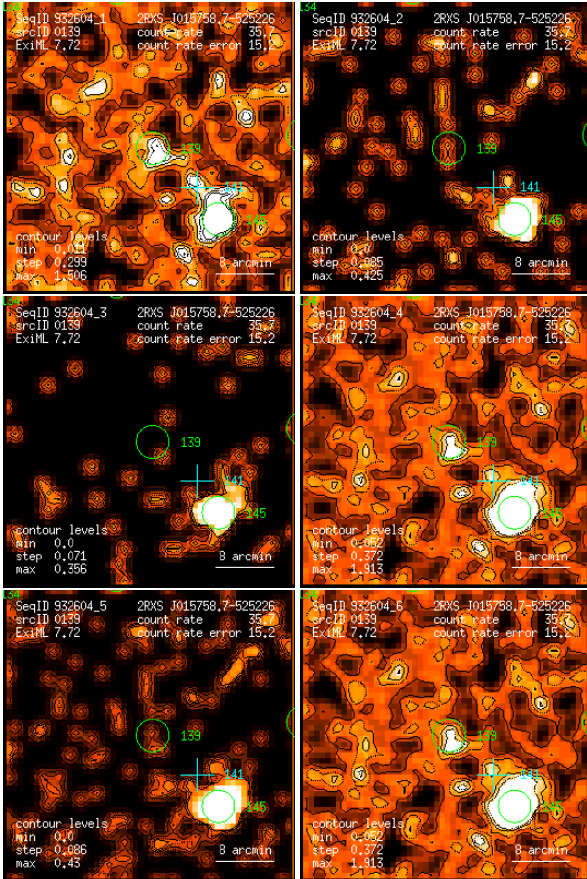
Figure 139: RASS 932604: detection 0139: band rate images, Gaussian filter: (1) PSPC channels 11 – 41, (2) 52 – 90, (3) 91 – 201, (4) 11 – 235, (5) 52 – 201, (6) 11 – 201. Broad band rates in counts/ks. Band rate contour levels in counts/ks/arcmin 2 .
