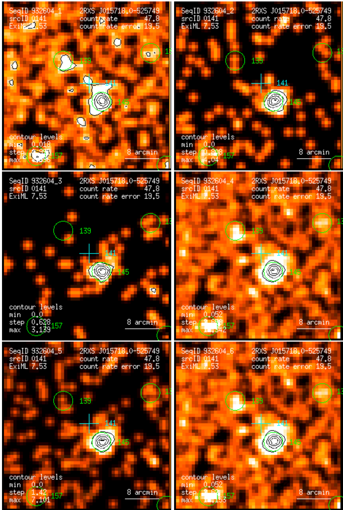
Figure 141: RASS 932604: detection 0141: band rate images, Gaussian filter: (1) PSPC channels 11 – 41, (2) 52 – 90, (3) 91 – 201, (4) 11 – 235, (5) 52 – 201, (6) 11 – 201. Broad band rates in counts/ks. Band rate contour levels in counts/ks/arcmin 2 .
