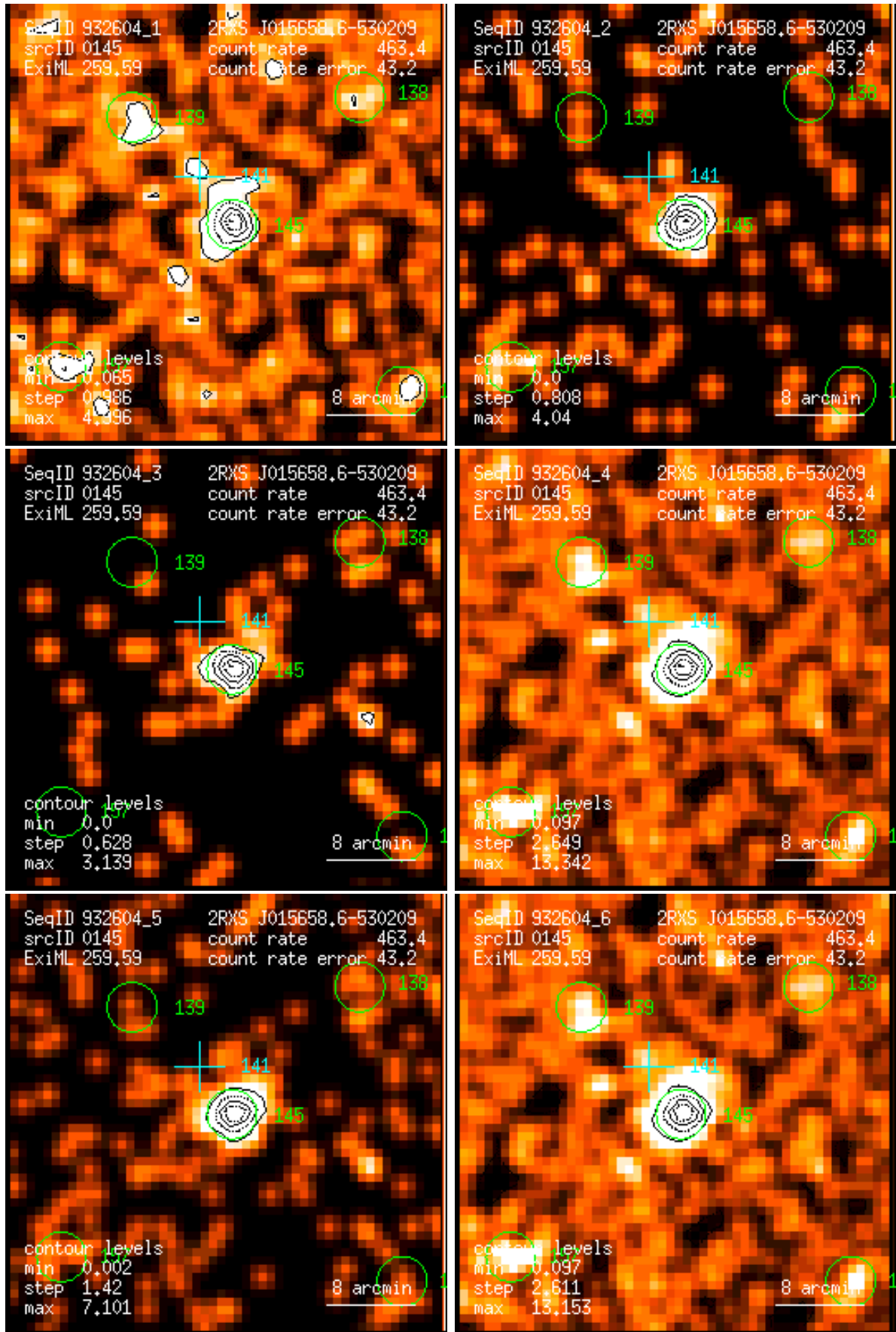
Figure 145: RASS 932604: detection 0145: band rate images, Gaussian filter: (1) PSPC channels 11 – 41, (2) 52 – 90, (3) 91 – 201, (4) 11 – 235, (5) 52 – 201, (6) 11 – 201. Broad band rates in counts/ks. Band rate contour levels in counts/ks/arcmin 2 .
