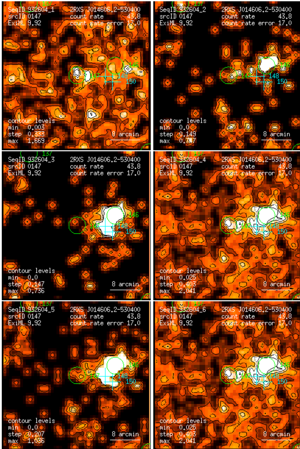
Figure 147: RASS 932604: detection 0147: band rate images, Gaussian filter: (1) PSPC channels 11 – 41, (2) 52 – 90, (3) 91 – 201, (4) 11 – 235, (5) 52 – 201, (6) 11 – 201. Broad band rates in counts/ks. Band rate contour levels in counts/ks/arcmin 2 .
