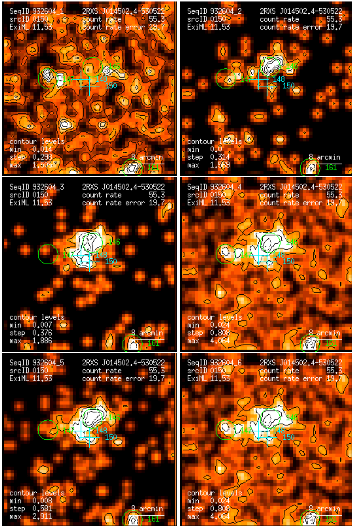
Figure 150: RASS 932604: detection 0150: band rate images, Gaussian filter: (1) PSPC channels 11 – 41, (2) 52 – 90, (3) 91 – 201, (4) 11 – 235, (5) 52 – 201, (6) 11 – 201. Broad band rates in counts/ks. Band rate contour levels in counts/ks/arcmin 2 .
