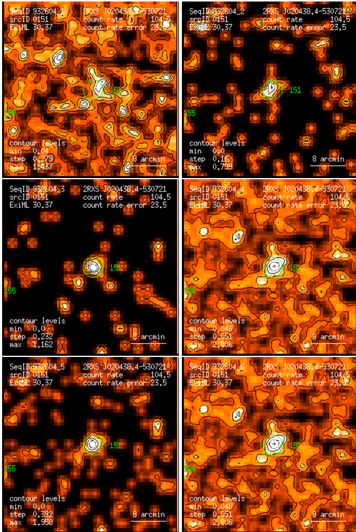
Figure 151: RASS 932604: detection 0151: band rate images, Gaussian filter: (1) PSPC channels 11 – 41, (2) 52 – 90, (3) 91 – 201, (4) 11 – 235, (5) 52 – 201, (6) 11 – 201. Broad band rates in counts/ks. Band rate contour levels in counts/ks/arcmin 2 .
