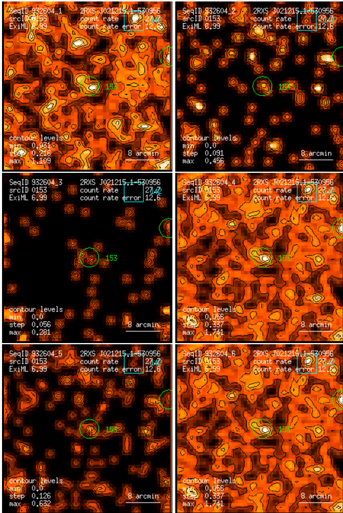
Figure 153: RASS 932604: detection 0153: band rate images, Gaussian filter: (1) PSPC channels 11 – 41, (2) 52 – 90, (3) 91 – 201, (4) 11 – 235, (5) 52 – 201, (6) 11 – 201. Broad band rates in counts/ks. Band rate contour levels in counts/ks/arcmin 2 .
