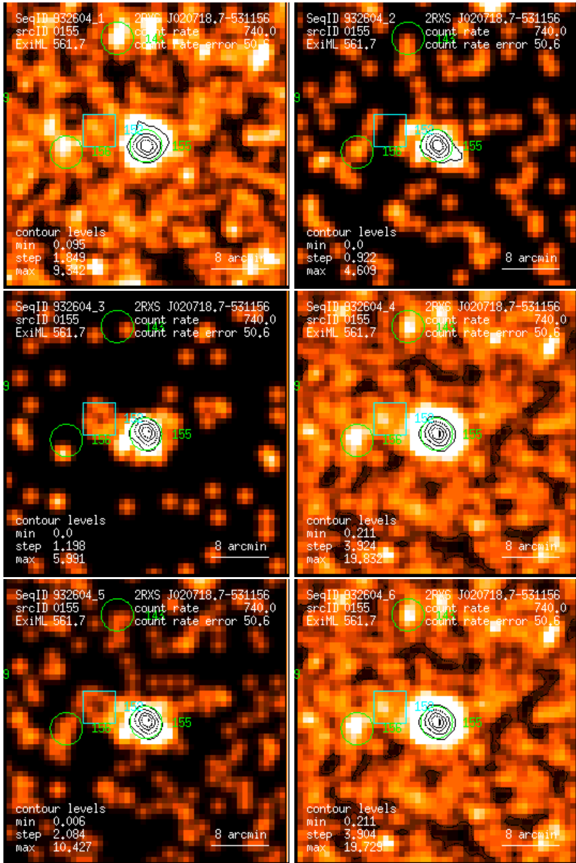
Figure 155: RASS 932604: detection 0155: band rate images, Gaussian filter: (1) PSPC channels 11 – 41, (2) 52 – 90, (3) 91 – 201, (4) 11 – 235, (5) 52 – 201, (6) 11 – 201. Broad band rates in counts/ks. Band rate contour levels in counts/ks/arcmin 2 .
