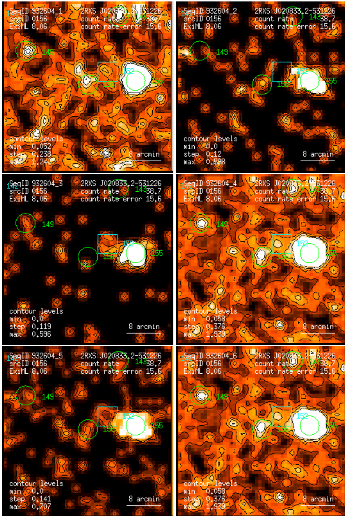
Figure 156: RASS 932604: detection 0156: band rate images, Gaussian filter: (1) PSPC channels 11 – 41, (2) 52 – 90, (3) 91 – 201, (4) 11 – 235, (5) 52 – 201, (6) 11 – 201. Broad band rates in counts/ks. Band rate contour levels in counts/ks/arcmin 2 .
