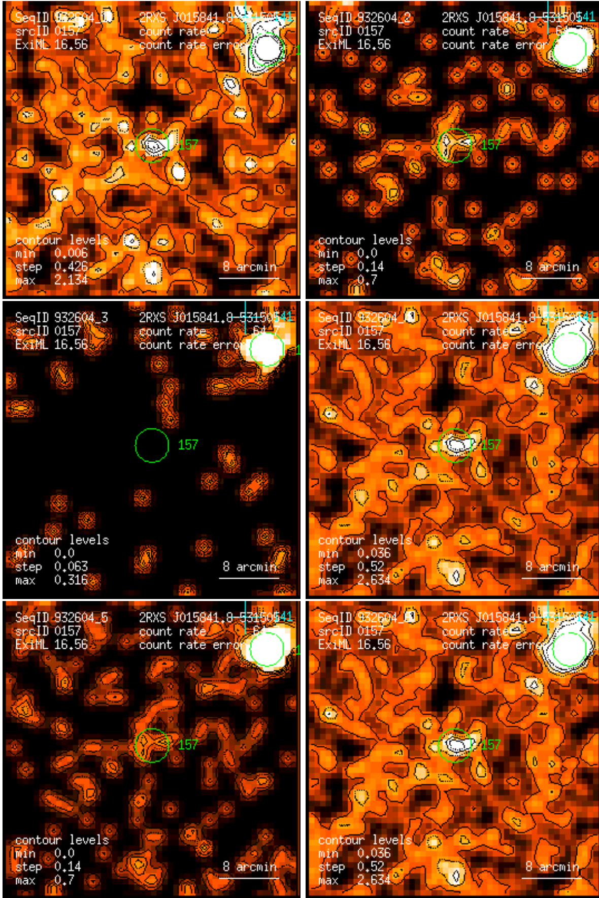
Figure 157: RASS 932604: detection 0157: band rate images, Gaussian filter: (1) PSPC channels 11 – 41, (2) 52 – 90, (3) 91 – 201, (4) 11 – 235, (5) 52 – 201, (6) 11 – 201. Broad band rates in counts/ks. Band rate contour levels in counts/ks/arcmin 2 .
