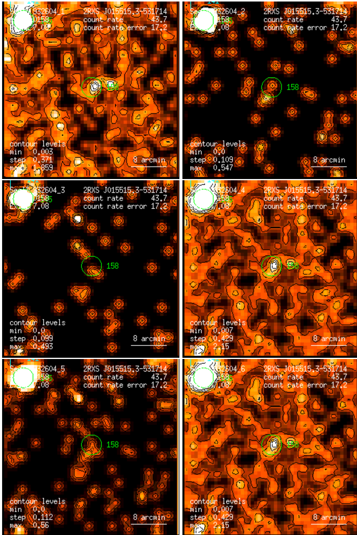
Figure 158: RASS 932604: detection 0158: band rate images, Gaussian filter: (1) PSPC channels 11 – 41, (2) 52 – 90, (3) 91 – 201, (4) 11 – 235, (5) 52 – 201, (6) 11 – 201. Broad band rates in counts/ks. Band rate contour levels in counts/ks/arcmin 2 .
