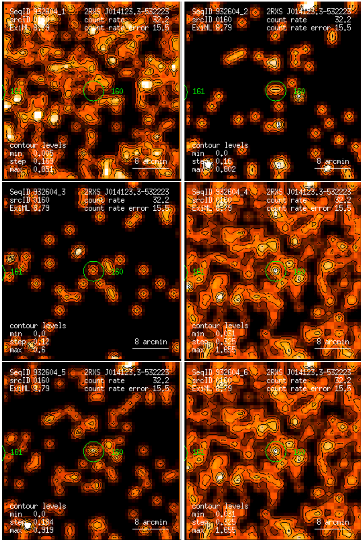
Figure 160: RASS 932604: detection 0160: band rate images, Gaussian filter: (1) PSPC channels 11 – 41, (2) 52 – 90, (3) 91 – 201, (4) 11 – 235, (5) 52 – 201, (6) 11 – 201. Broad band rates in counts/ks. Band rate contour levels in counts/ks/arcmin 2 .
