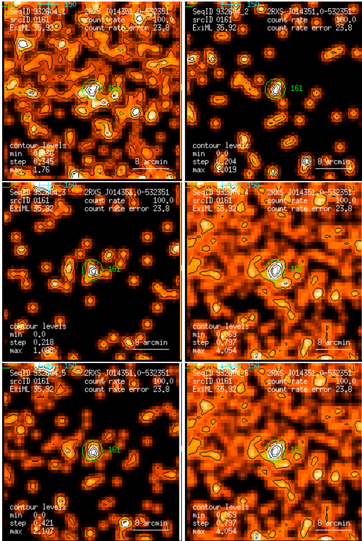
Figure 161: RASS 932604: detection 0161: band rate images, Gaussian filter: (1) PSPC channels 11 – 41, (2) 52 – 90, (3) 91 – 201, (4) 11 – 235, (5) 52 – 201, (6) 11 – 201. Broad band rates in counts/ks. Band rate contour levels in counts/ks/arcmin 2 .
