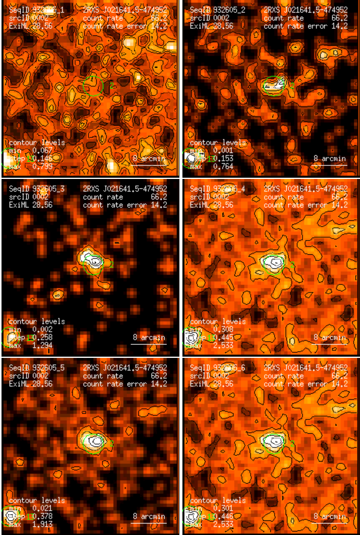
Figure 2: RASS 932605: detection 0002: band rate images, Gaussian filter: (1) PSPC channels 11 – 41, (2) 52 – 90, (3) 91 – 201, (4) 11 – 235, (5) 52 – 201, (6) 11 – 201. Broad band rates in counts/ks. Band rate contour levels in counts/ks/arcmin 2 .
