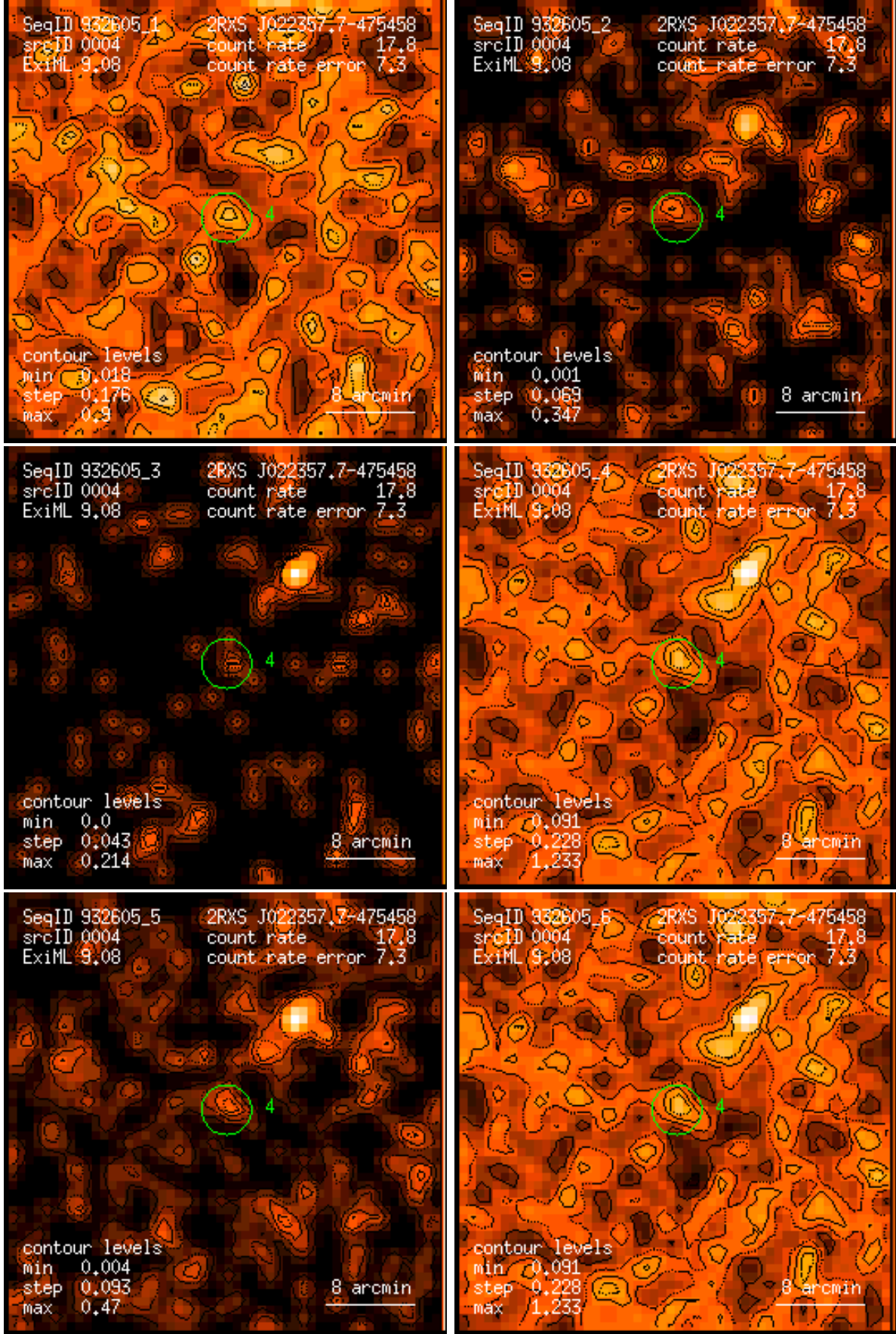
Figure 4: RASS 932605: detection 0004: band rate images, Gaussian filter: (1) PSPC channels 11 – 41, (2) 52 – 90, (3) 91 – 201, (4) 11 – 235, (5) 52 – 201, (6) 11 – 201. Broad band rates in counts/ks. Band rate contour levels in counts/ks/arcmin 2 .
