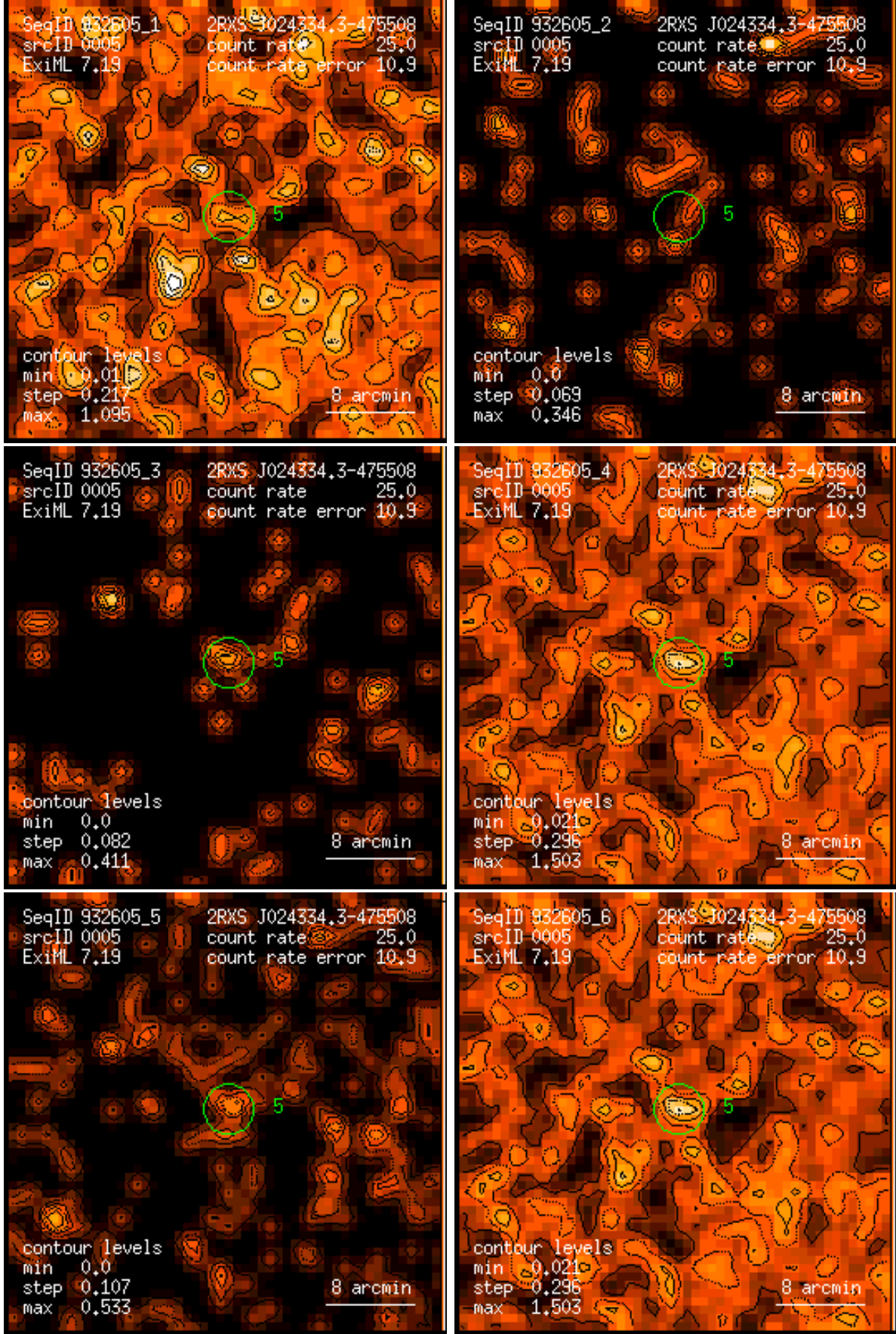
Figure 5: RASS 932605: detection 0005: band rate images, Gaussian filter: (1) PSPC channels 11 – 41, (2) 52 – 90, (3) 91 – 201, (4) 11 – 235, (5) 52 – 201, (6) 11 – 201. Broad band rates in counts/ks. Band rate contour levels in counts/ks/arcmin 2 .
