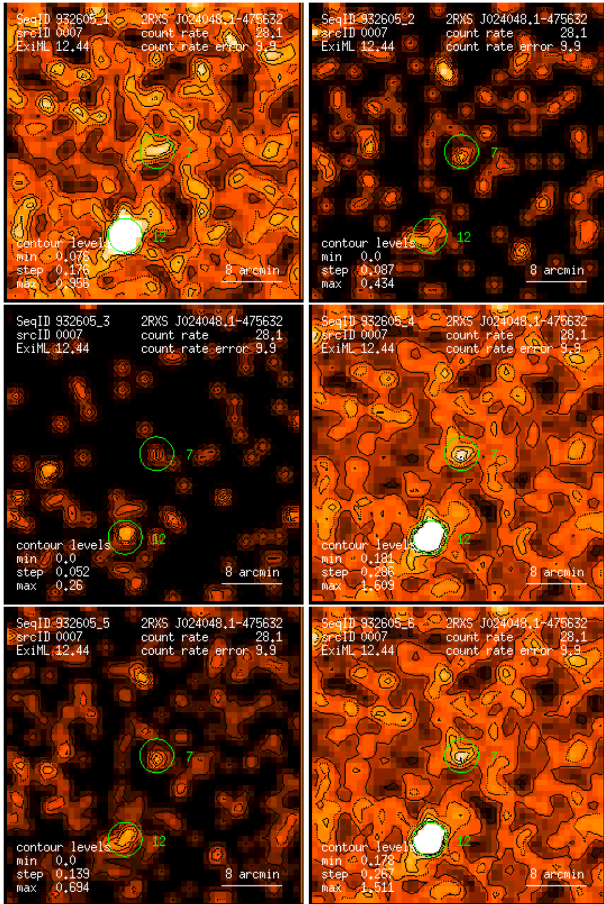
Figure 7: RASS 932605: detection 0007: band rate images, Gaussian filter: (1) PSPC channels 11 – 41, (2) 52 – 90, (3) 91 – 201, (4) 11 – 235, (5) 52 – 201, (6) 11 – 201. Broad band rates in counts/ks. Band rate contour levels in counts/ks/arcmin 2 .
