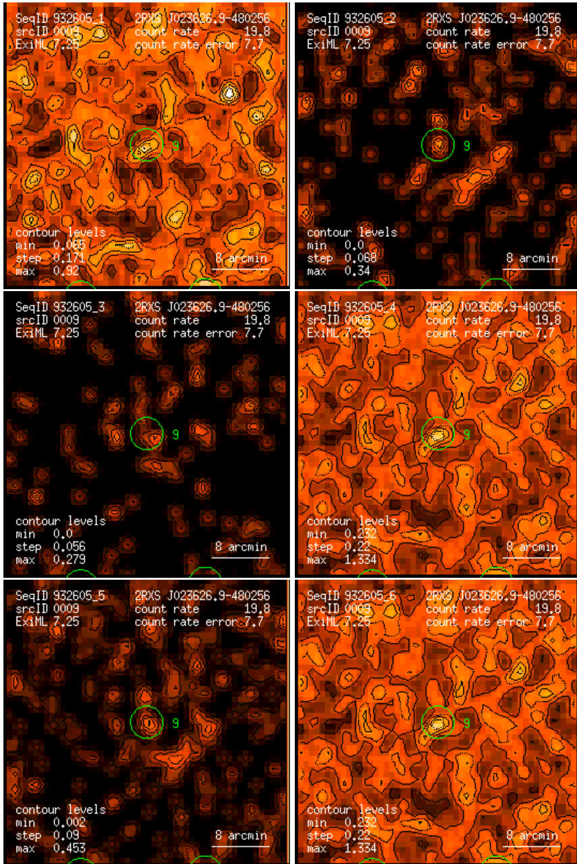
Figure 9: RASS 932605: detection 0009: band rate images, Gaussian filter: (1) PSPC channels 11 – 41, (2) 52 – 90, (3) 91 – 201, (4) 11 – 235, (5) 52 – 201, (6) 11 – 201. Broad band rates in counts/ks. Band rate contour levels in counts/ks/arcmin 2 .
