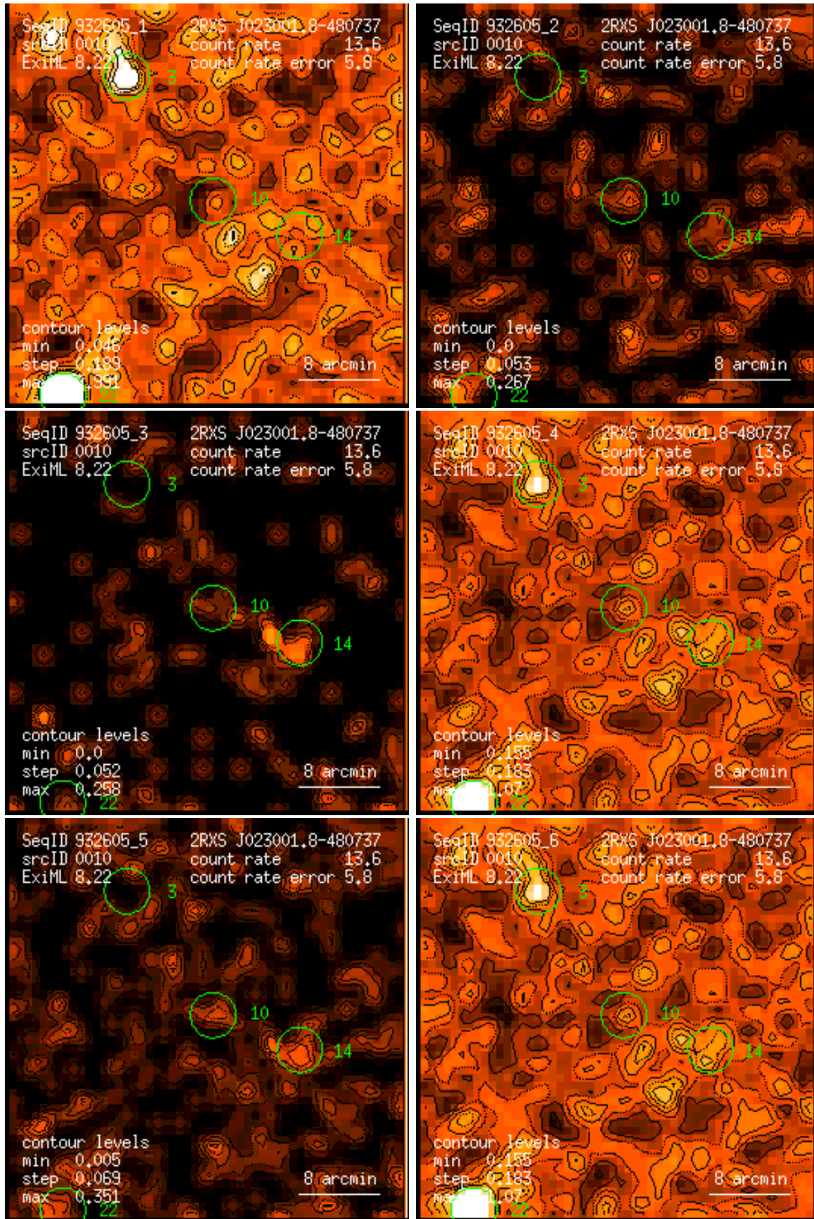
Figure 10: RASS 932605: detection 0010: band rate images, Gaussian filter: (1) PSPC channels 11 – 41, (2) 52 – 90, (3) 91 – 201, (4) 11 – 235, (5) 52 – 201, (6) 11 – 201. Broad band rates in counts/ks. Band rate contour levels in counts/ks/arcmin 2 .
