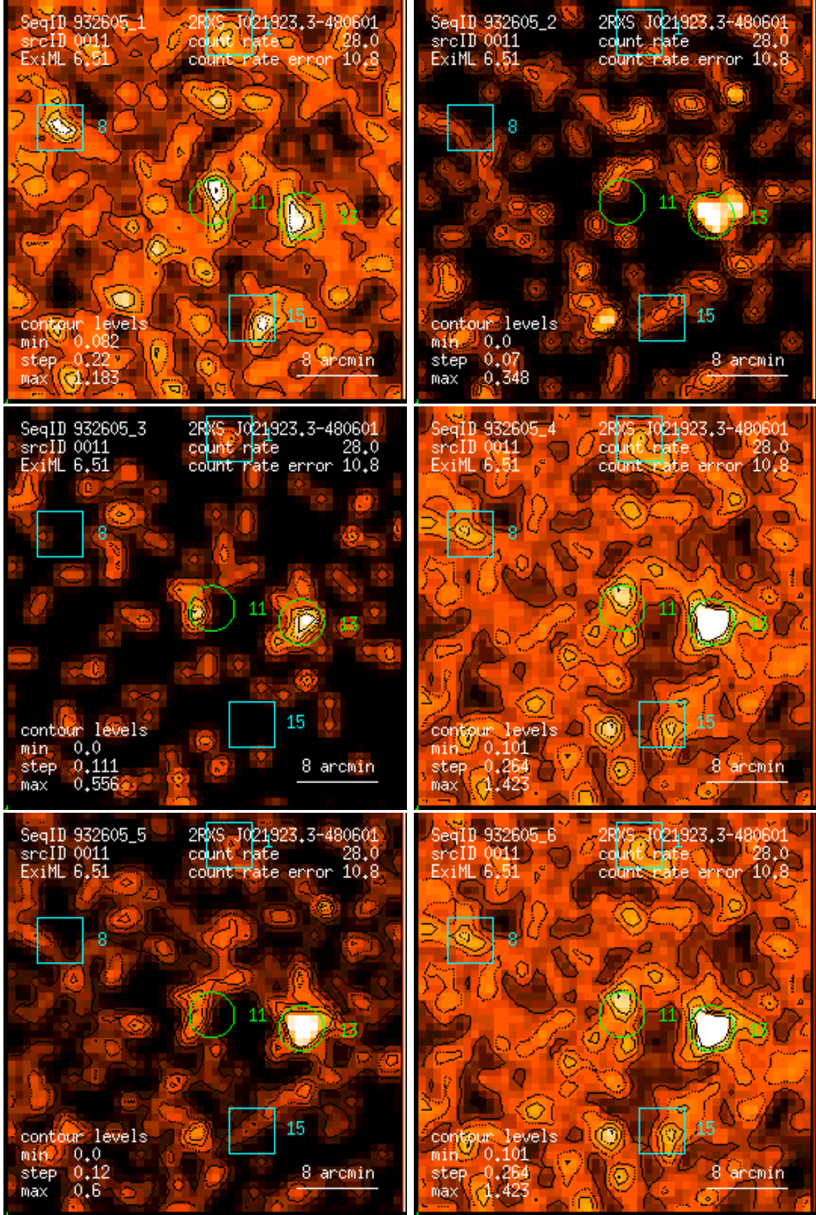
Figure 11: RASS 932605: detection 0011: band rate images, Gaussian filter: (1) PSPC channels 11 – 41, (2) 52 – 90, (3) 91 – 201, (4) 11 – 235, (5) 52 – 201, (6) 11 – 201. Broad band rates in counts/ks. Band rate contour levels in counts/ks/arcmin 2 .
