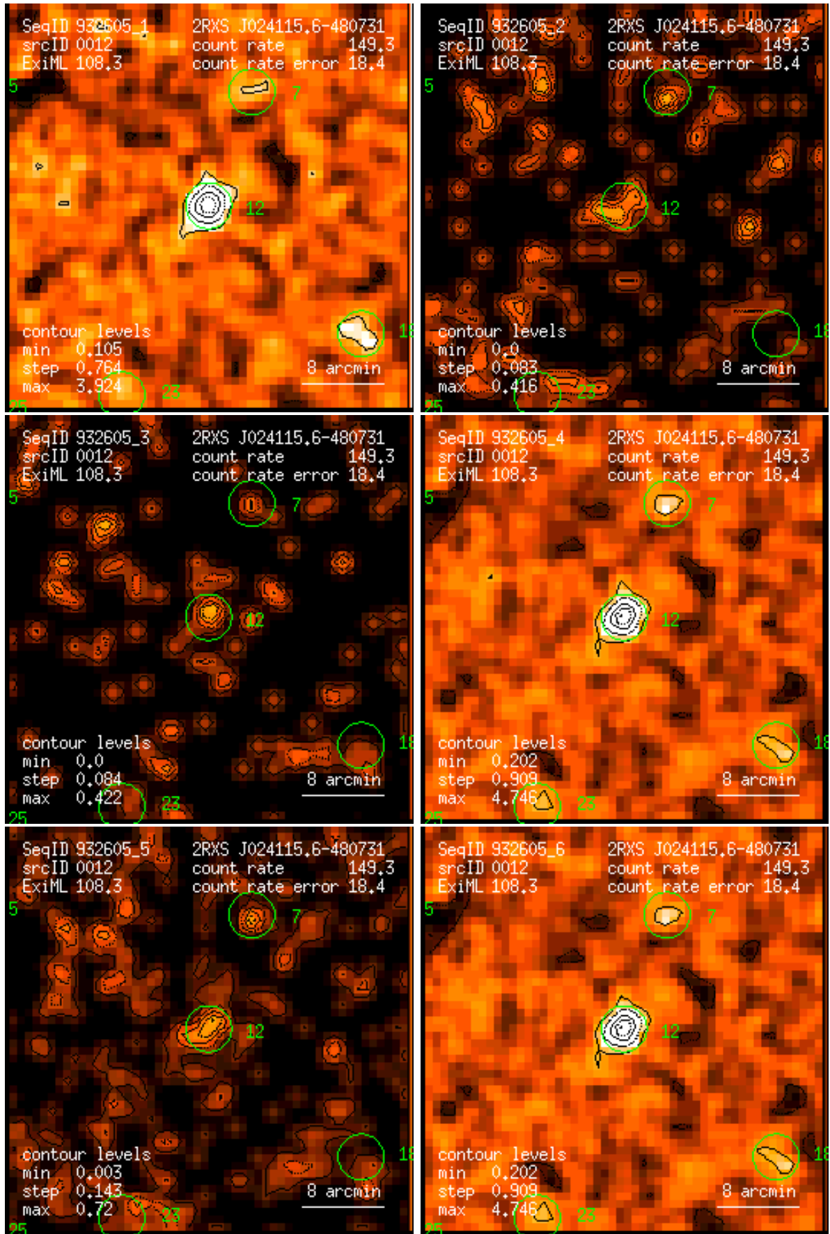
Figure 12: RASS 932605: detection 0012: band rate images, Gaussian filter: (1) PSPC channels 11 – 41, (2) 52 – 90, (3) 91 – 201, (4) 11 – 235, (5) 52 – 201, (6) 11 – 201. Broad band rates in counts/ks. Band rate contour levels in counts/ks/arcmin 2 .
