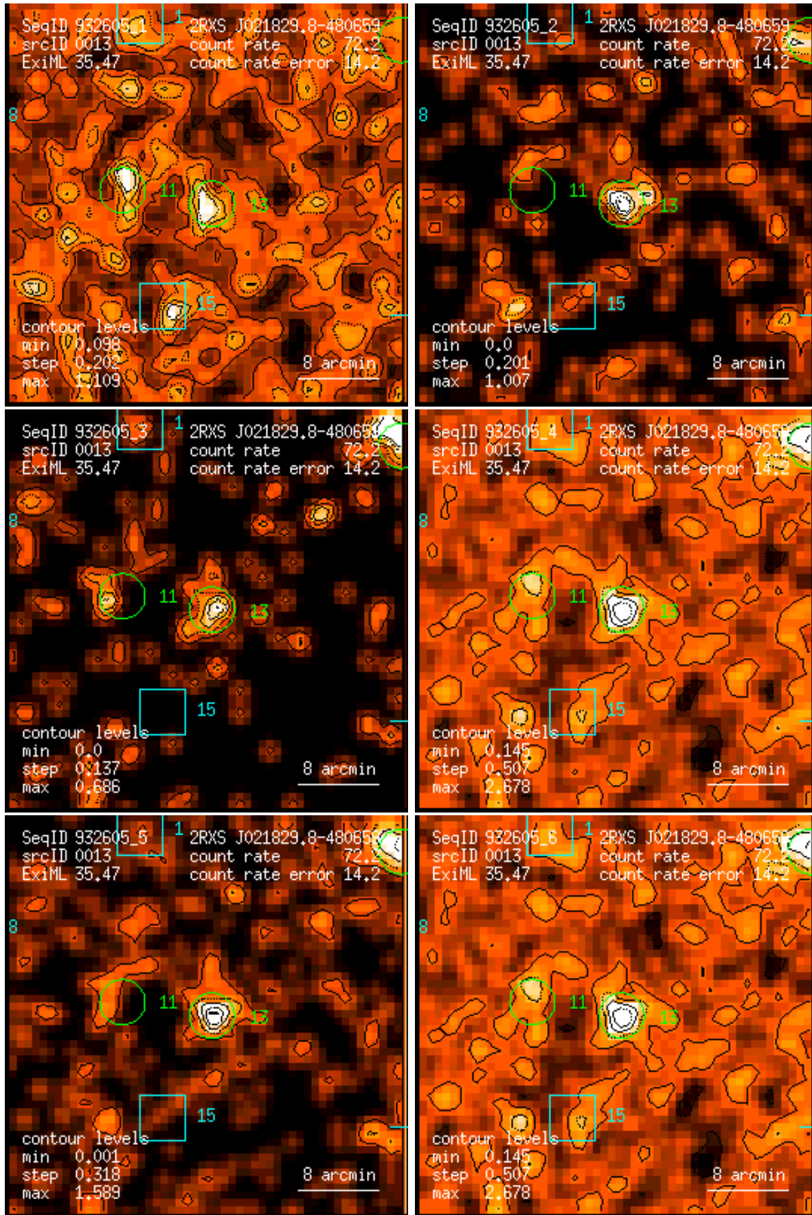
Figure 13: RASS 932605: detection 0013: band rate images, Gaussian filter: (1) PSPC channels 11 – 41, (2) 52 – 90, (3) 91 – 201, (4) 11 – 235, (5) 52 – 201, (6) 11 – 201. Broad band rates in counts/ks. Band rate contour levels in counts/ks/arcmin 2 .
