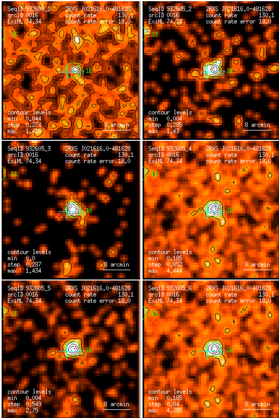
Figure 16: RASS 932605: detection 0016: band rate images, Gaussian filter: (1) PSPC channels 11 – 41, (2) 52 – 90, (3) 91 – 201, (4) 11 – 235, (5) 52 – 201, (6) 11 – 201. Broad band rates in counts/ks. Band rate contour levels in counts/ks/arcmin 2 .
